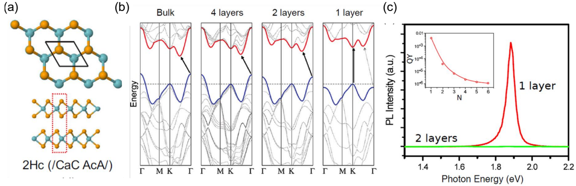
Figure 1.10: Crystalline structure of TMDs. (a) Top and bottom view of the 2Hc polytype. The primitive unit cell is shown with the diamond in the top view and the square box in the side view. Figure adapted from [56] (b) Calculated band structure from bulk to monolayer MoS 2 showing the indirect-to-direct bandgap transition at the K point. Figure adapted from [57]. The arrows show the lowest energetic transition (c) Photoluminescence spectra recorded at 300K on mono and bilayer MoS 2 . The inset shows the quantum emission yield as a function of the number of layers. Figure adapted from [58]
