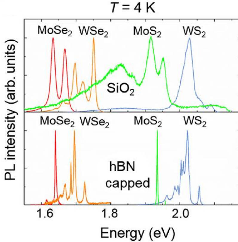
Figure 1.9: Approaching the homogeneous limit with hBN. Top: PL spectra of MoSe 2 , WSe 2 , MoS 2 and WS 2 deposited on SiO 2 taken at 4K. Bottom: PL spectra of hBN-capped MoSe 2 , WSe 2 , MoS 2 and WS 2 taken at 4K. We can see the optical quality improvement of the TMDs through the sharpening of the emission peaks. Indeed, this is a sign of a reduction of environmental disorder. Figure extracted from [55].
