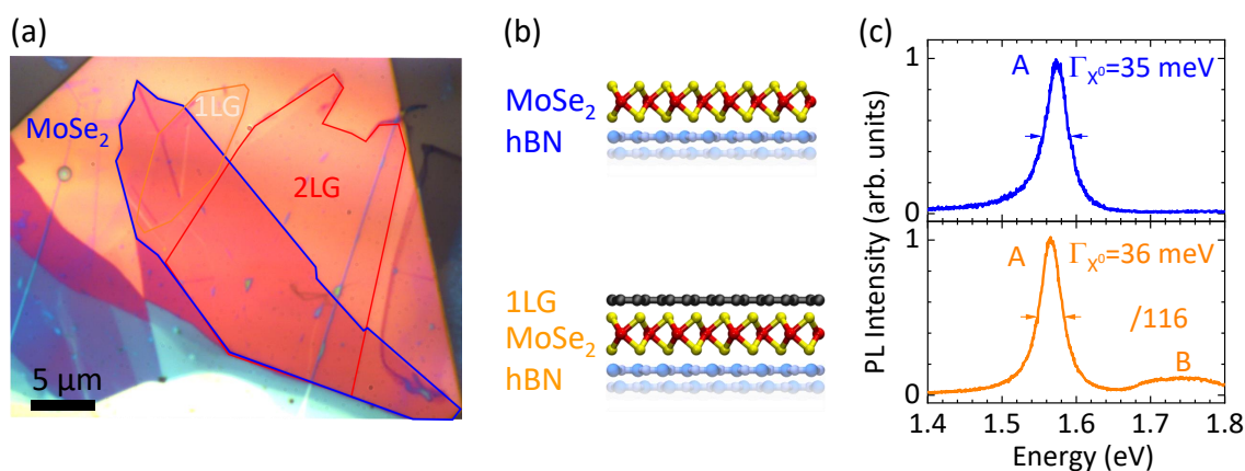
Figure 3.1: hBN-supported MoSe 2 /1LG sample. (a) Optical microscopy image of a hBN/MoSe 2 /1-2LG sample. (b) Lateral view of the sample. (c) Room temperature PL spectra of hBN/MoSe 2 (top) and hBN/MoSe 2 /1LG (bottom). The FWHM of the peaks is indicated in the figure. Spectra recorded with a 532 nm cw-laser with an intensity of 1 \mu\text{W}/\mu\text{m}^2 .
