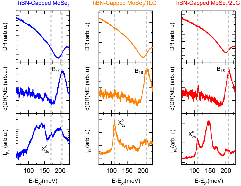
Figure 3.15: Dielectric screening and reduced binding energy in hBN-capped MoSe 2 /1LG From top to bottom: DR, d(\text{DR})/dE and I_{PL} spectra of hBN-capped MoSe 2 (blue), hBN-capped MoSe 2 /1LG (orange) and hBN-capped MoSe 2 /2LG (red). PL Spectra recorded at 14K under cw excitation at 633 nm and 100 \mu\text{W}/\mu\text{m}^2 .
