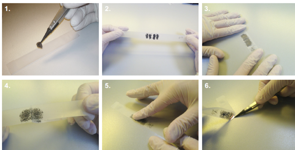
Figure 2.1: Scheme of the exfoliation process. (1) A bulk crystal is put onto a scotch tape. (2) The scotch tape is folded over the crystal and peeled off afterward. (3) A second scotch tape is put on top of the first one. (4) The second scotch tape is peeled off and the same procedure is repeated until transparent areas of the crystal appear. (5) The scotch tape is placed onto the target substrate. (6) Carefully peel off the scotch tape. Figure extracted from [38]
