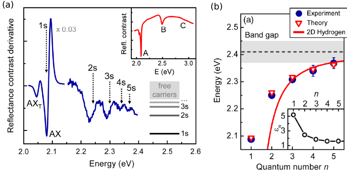
Figure 1.15: Non-hydrogenic Rydberg series. (a) Derivative of the reflectance contrast for monolayer WS 2 on SiO 2 . The 1s A-exciton is visible as well as its corresponding Rydberg series up to the 5s state. The inset shows the full spectra and the absorption line corresponding to the B-exciton as well. (b) Experimental and theoretical values of the transition energies as a function of the quantum number. The 2D-H model is not sufficient to explain the behavior at low n . The inset shows the effective screening as a function of the quantum number n . Figures adapted from [77].
