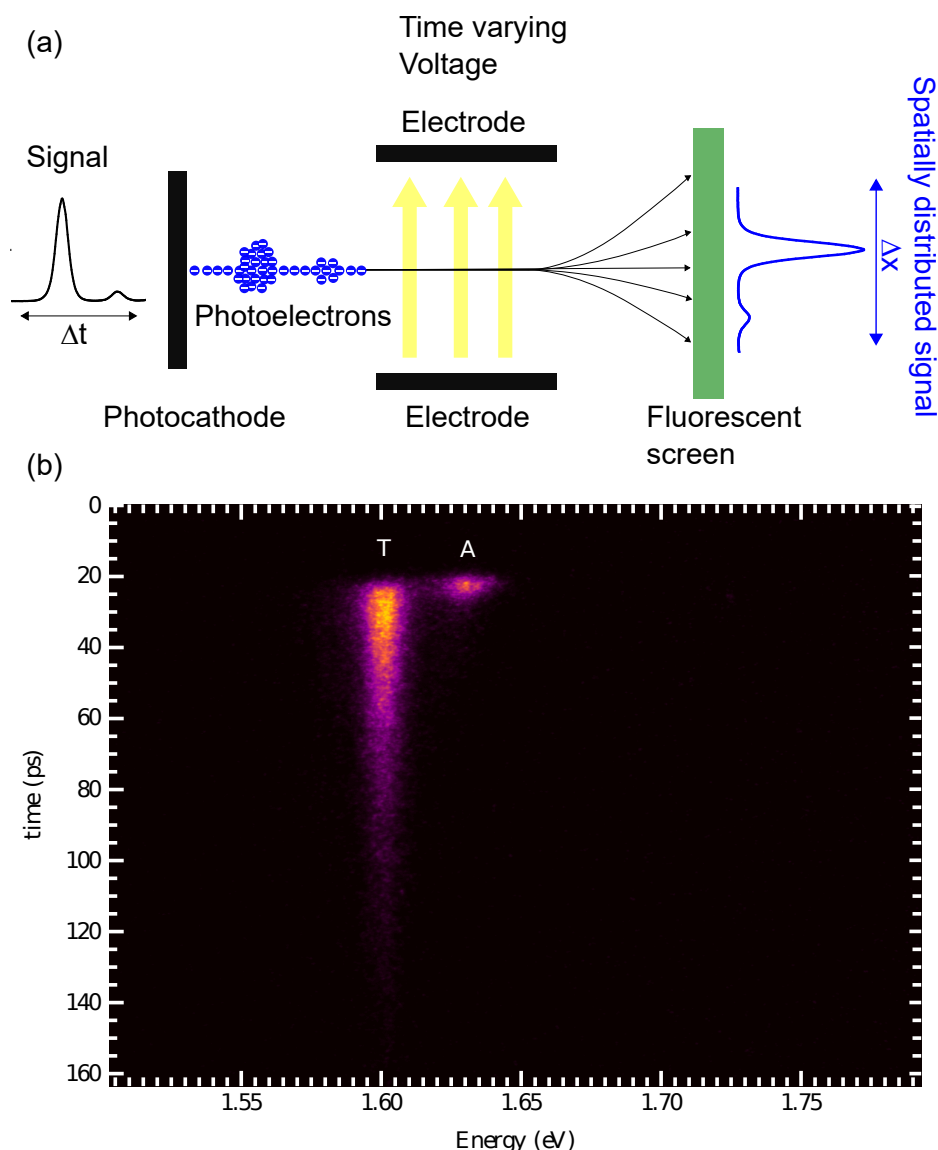
Figure 2.10: Streak camera working principle. (a) Scheme of the working principle of a streak camera. (b) Streak image of a monolayer MoSe 2 at 4 K. A and T denote the exciton and trion respectively. Figure (b) was extracted from [71]
