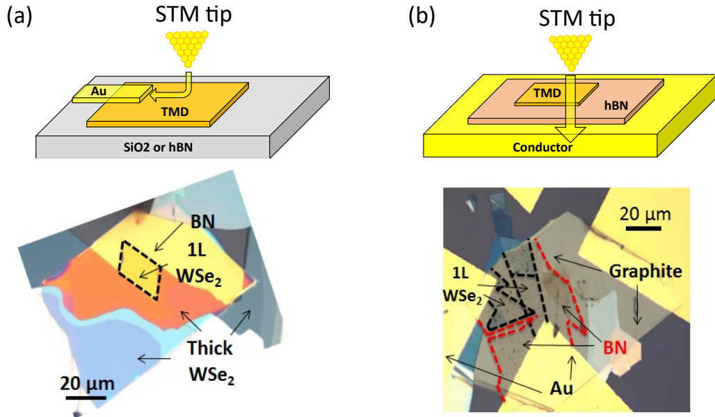
Figure B.1: STM-compatible samples. (a) Top: Scheme of a lateral configuration. The current travels along the sample. Bottom: optical image of monolayer \text{WSe}_2 on hBN. This sample was later contacted with gold as shown in the top scheme. (b) Top: Scheme of a vertical transport configuration. Bottom: Optical image of monolayer \text{WSe}_2 on graphite with a few layers of hBN as a decoupling element.
