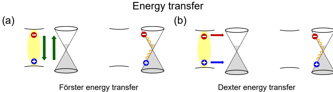
Figure 3.6: Energy transfer mechanism. Scheme illustrating the energy transfer process. (a) FRET process in which an exciton in the TMD transfer its energy to graphene through dipole-dipole interaction (b) DET process in which an exciton in the TMD tunnels into graphene. Both processes end up in the same final state.
