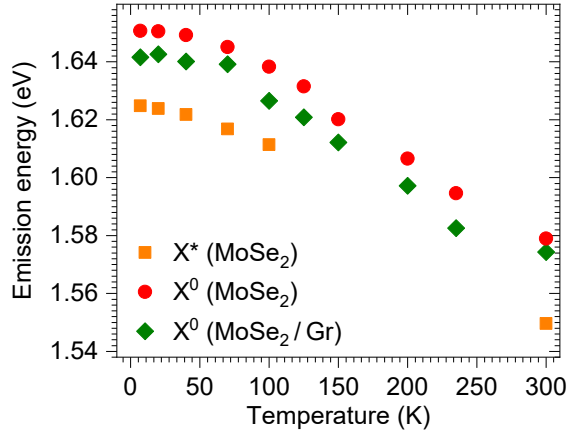
Figure 3.11: Temperature dependent PL spectroscopy on a hBN-capped MoSe 2 /1LG sample . Temperature dependent peak energy of the MoSe 2 exciton ( X^0 ) and trion ( X^* ) emission lines. All data were recorded in the linear regime using cw-laser excitation at 2.33 eV.
