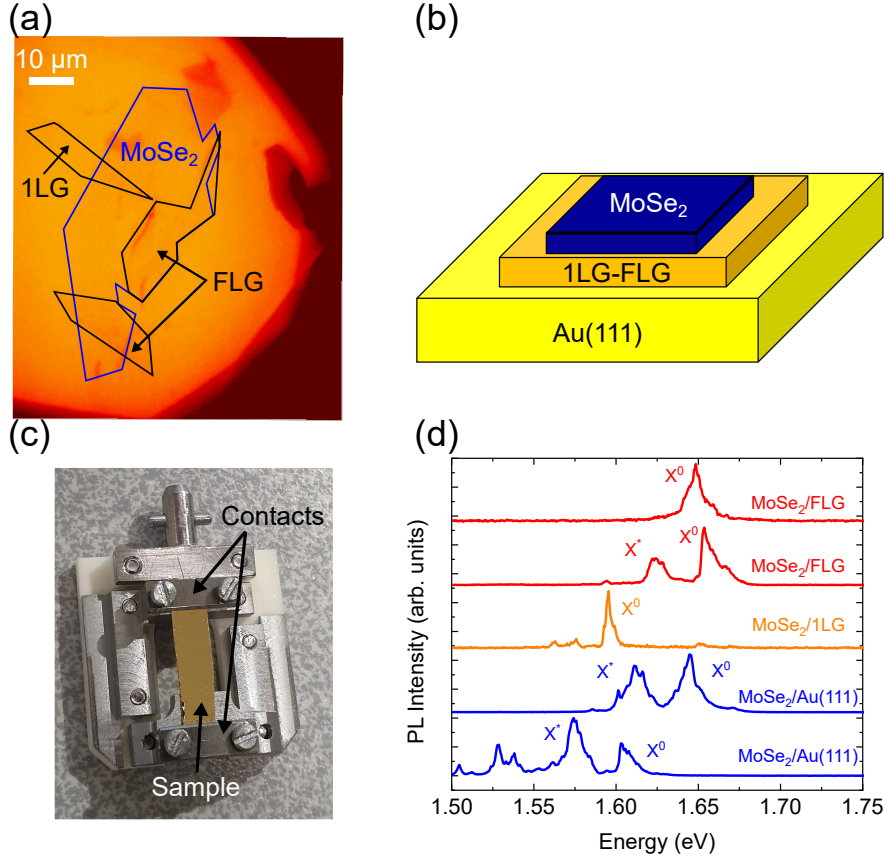
Figure 4.5: Characterization of the sample. (a) Optical microscopy image of a monolayer \text{MoSe}_2/\text{FLG} deposited onto a \text{Au}(111) film on mica. (b) Graphical representation of the sample architecture. (c) Image of the sample holder. (d) Normalized PL spectra acquired in different regions of the sample. For each spectra the X^0 and X^* are signaled. The PL measurements were done under cw excitation at 532 nm under a laser power of 60 \mu\text{W}/\mu\text{m}^2 and at 14 K.
