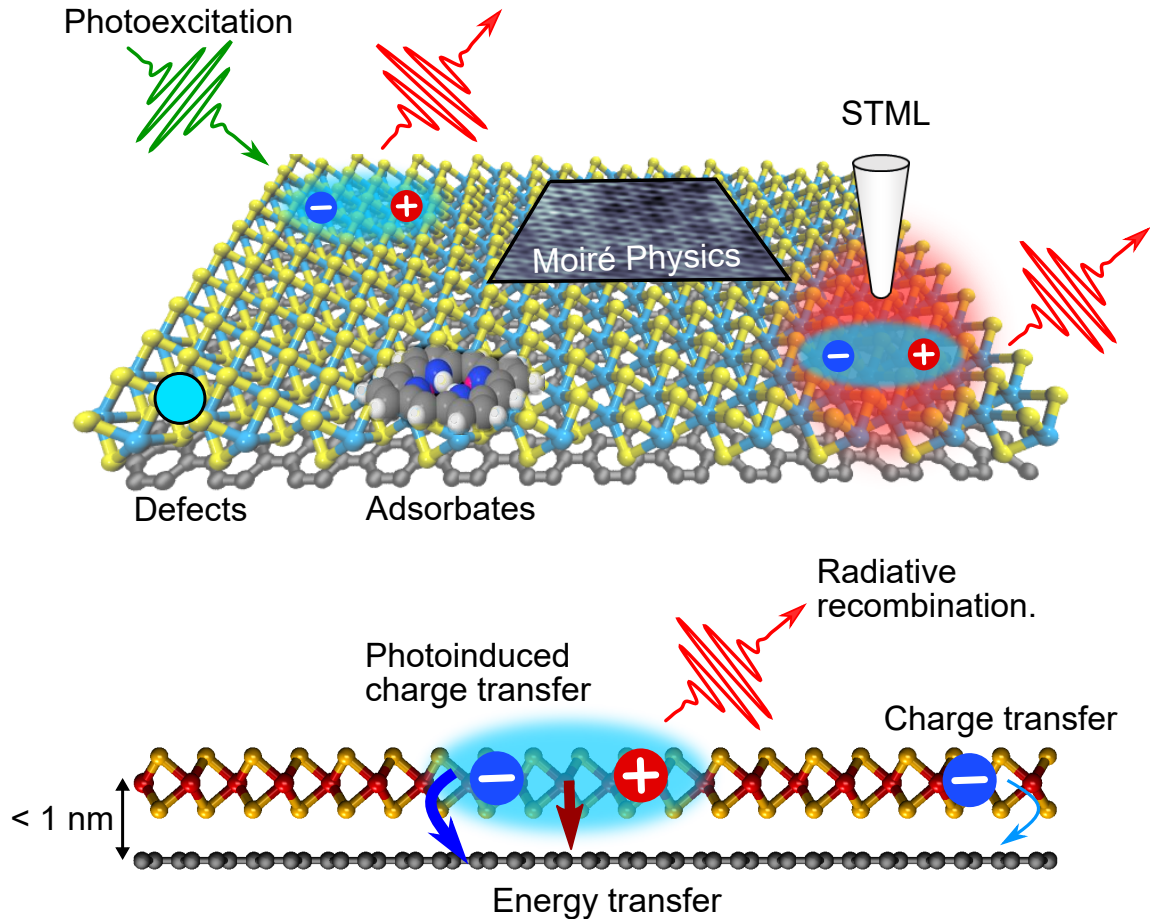
Figure 12: Tailoring the luminescence of atomically thin semiconductors at the sub-nm scale. Top: 3D-scheme of a monolayer TMD/graphene heterostructure. Exciton generation occurs either through photoexcitation (green wavy arrow) or using an STM current. We can identify the different nanoscopic environments an exciton can experience. These are defects, adsorbates and Moiré patterns among others. Bottom: Interlayer coupling mechanisms that can arise at the interface of the heterostructure. These are charge transfer, energy transfer and electron redistribution.
