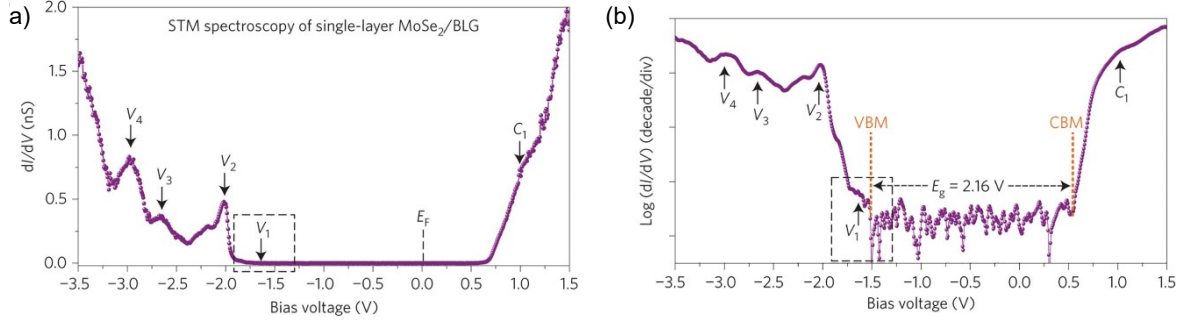
Figure 1.21: Electronic bandgap determination. (a) dI/dV spectra of a \text{MoSe}_2/\text{BLG} sample. We can see four resonances in the negative side arising from different bands being probed (b) Zoom on the dI/dV spectra showing the determination of the bandgap. Figures b-d extracted from [26]
