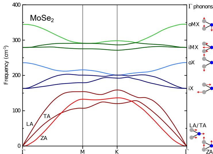
Figure 1.14: Vibrational properties of TMDs. Phonon dispersion relation calculated for MoSe 2 monolayer. The diagrams on the right hand side of the graph represent the atomic displacement associated with each phonon mode. Figure extracted from [71] (original data from [72]).
