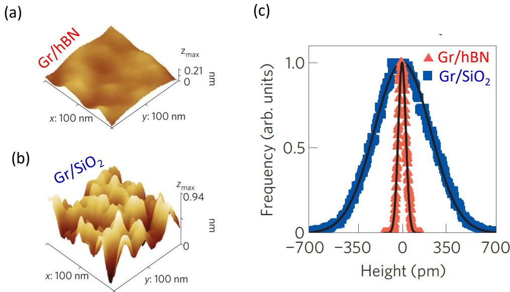
Figure 1.8: STM image of hBN- (a) and \text{SiO}_2 -supported graphene (b). hBN provides a flatter substrate on which graphene can accommodate. (c) Histogram comparing the height variations of hBN/Gr and hBN/ \text{SiO}_2 samples. Figure adapted from [53].
