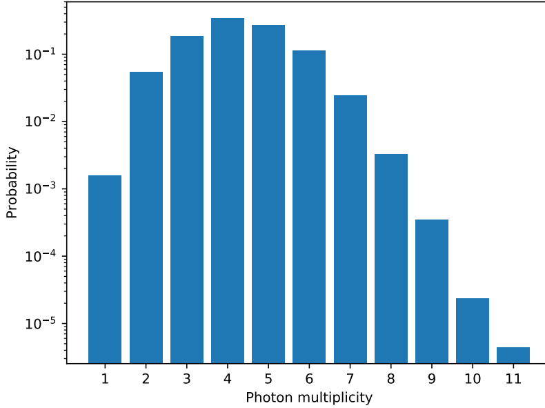
Figure 4.3: DICEBOX photon multiplicity distribution for ^{95}\text{Mo}(\text{n},\gamma) .
