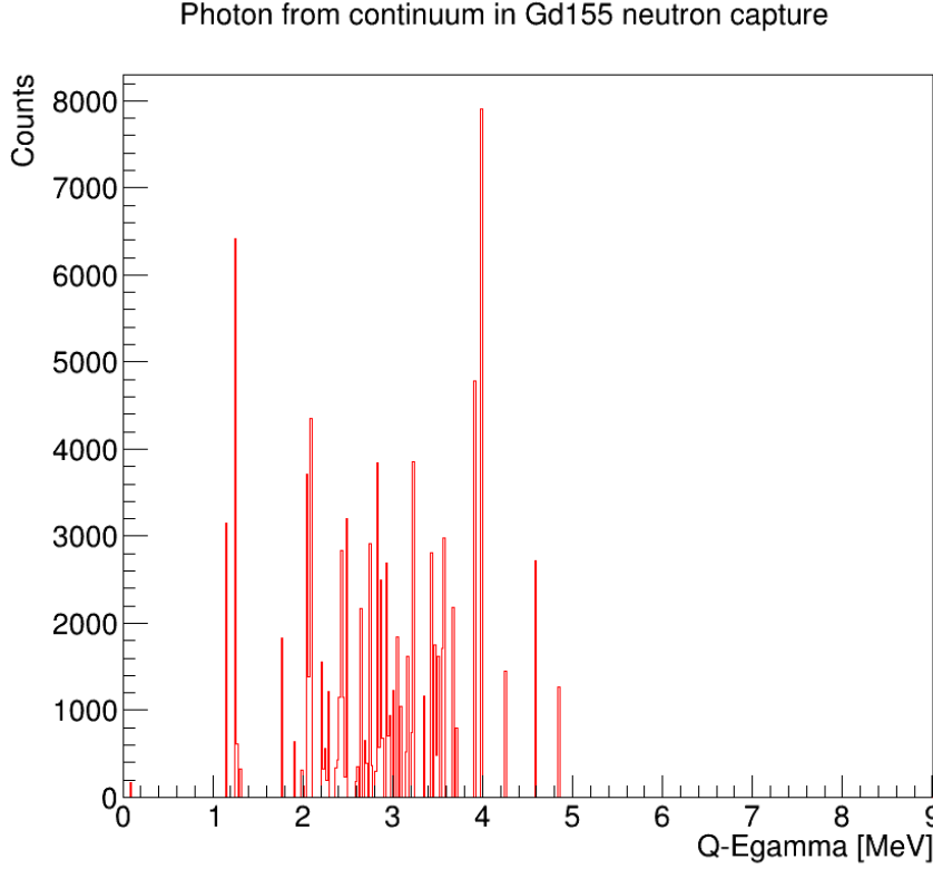
Figure 4.14: Excited states reached at first photon emission in ^{155}\text{Gd}(n,\gamma) PHITS simulation.
