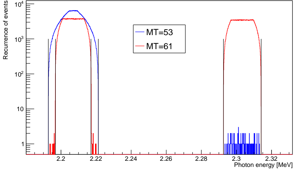
Figure 3.9: PHITS simulations with enhanced probabilities of reaching either the 3 rd or the 11 th excited state of ^{27}\text{Al} . The calculated kinematical limits are indicated by vertical black lines.
