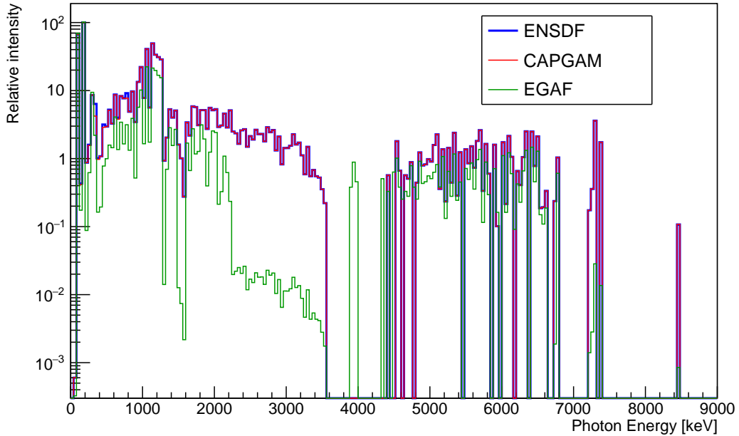
Figure 4.12: Thermal capture data for ^{155}\text{Gd} . The data are normalized with respect to the highest emission peak. (Violet-ish tone indicates perfect agreement between ENSDF and CAPGAM).
