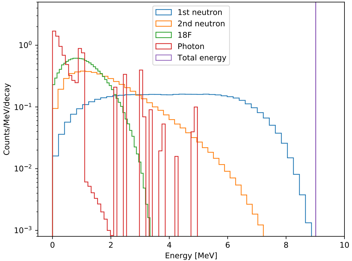
Figure 5.2: Total energy is conserved when the sampling of MF=6 MT=16 is done considering a decrease in available energy at each sampling for the ^{19}\text{F}(\text{n},2\text{n}) reaction.
