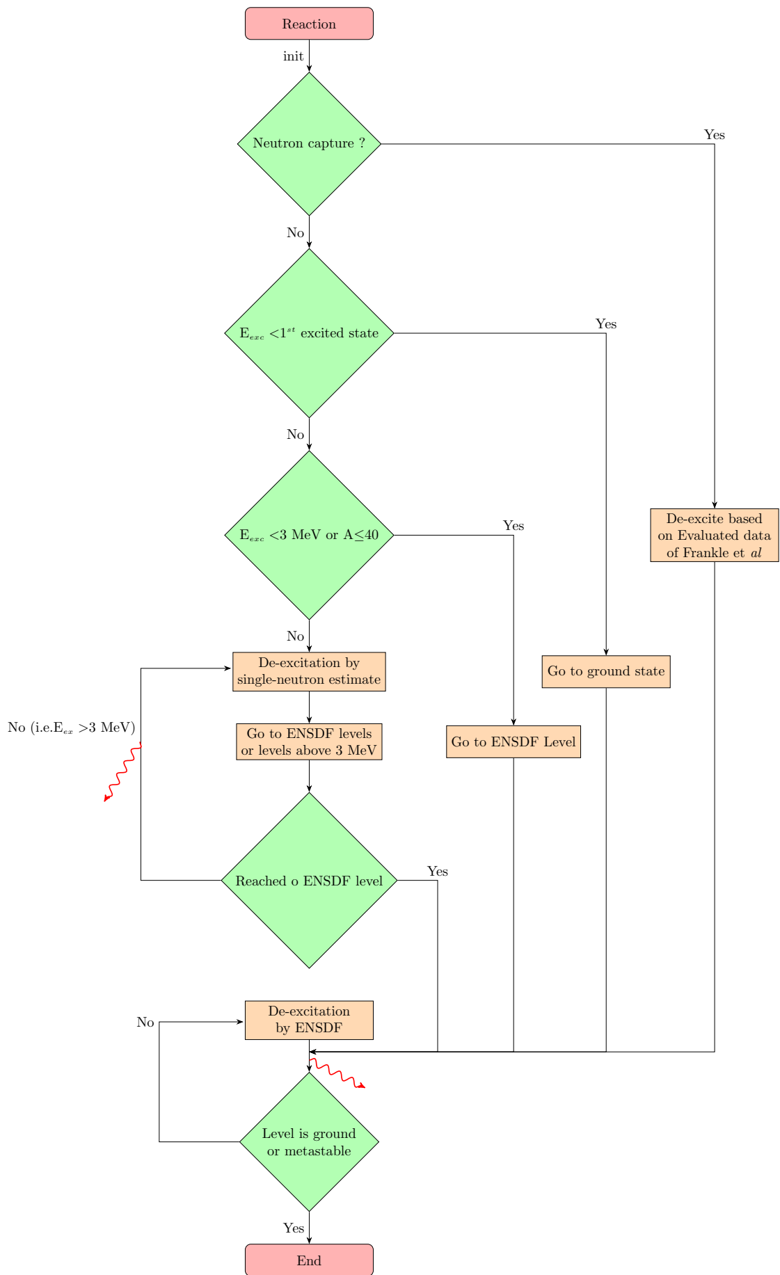
Figure 2.9: Algorithm of EBITEM. E_{ex} and A denote the excitation energy and mass number, respectively. Flow chart taken from ref. [1].
