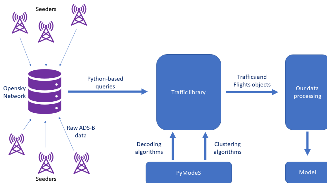
Figure 4.1: Architecture of the data processing
