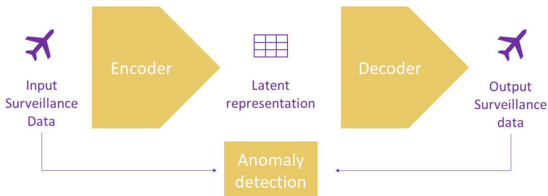
Figure 1.4: Basic architecture of a classic autoencoder for anomaly detection
