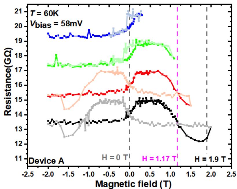
FIGURE 8.3: R(H) data for device-A Fe/CoPc(20nm)/Co measured at 60K and 58mV. Minor (blue, green, red) and major (black) R(H) loops show three resistance levels at H = 0\text{T} (gray), H = 1.17\text{T} (magenta) and H = 1.9\text{T} (black). The return cycle of the field sweep i.e., from H = +2\text{T} to -2\text{T} of the R(H) is given by the gray, light colors of red, green and blue.
