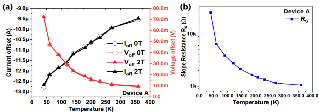
FIGURE 9.10: Temperature and magnetic field dependence of (I, V) offsets and slope resistance R_s . (a) Temperature has a strong impact on both I_{\text{off}} and V_{\text{off}} values unlike the magnetic field which has rather negligible effect on the (I, V) offsets. The circles represent the offsets at H = 0T and solid triangles are for H = 2T for 40 < T(K) < 360 . (b) Slope resistance R_s calculated for 40 < T(K) < 360 at H = 0T . For rising temperatures the resistance falls down i.e., at 40K (360K) the R_s is calculated to be 25.9k\Omega ( 1.05k\Omega ).
