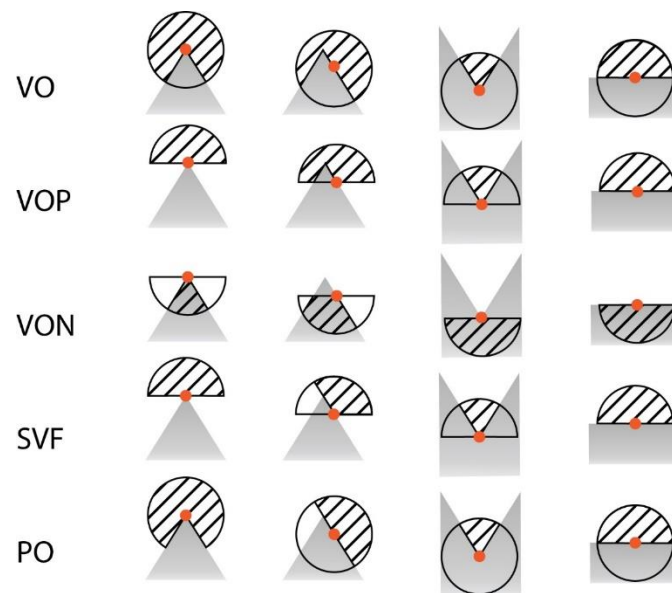
Figure 6. Sketches where hatching depicts the zones taken into account by the VO, VOP, VON, SVF, and PO methods, applied to different topographic cases.
