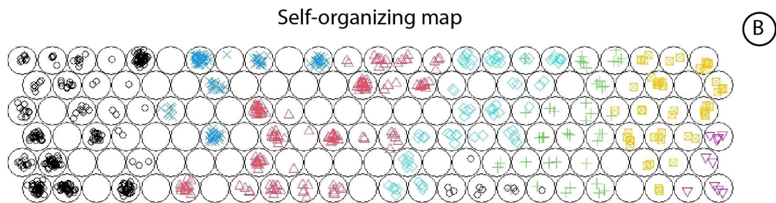
Fig. 8 A) Silhouette plot of the k=7 clusters. B) projection of the 790 individuals on the Self-organizing map. The clusters 1-7 are depicted with different colours and symbols. 1) black circles; 2) pink triangles; 3) green plus signs; 4) blue crosses; 5) light blue diamonds; 6) purple inverted triangles; 7) yellow squares.
