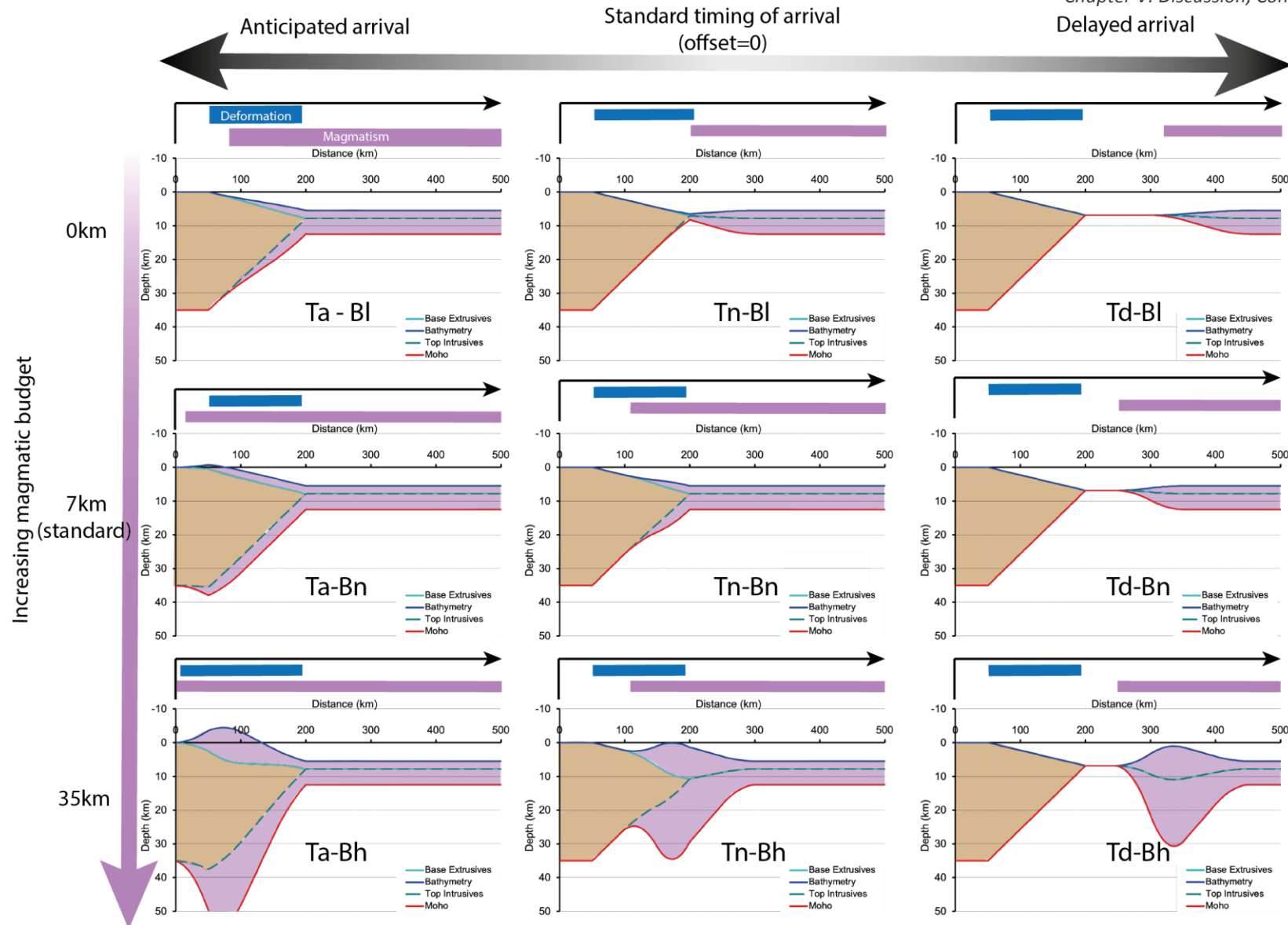
Figure 39: Represented, thermally equilibrated margin shapes based on different budgets and timing in magma production. Top horizontal axis represents the relative timing of arrival of magmatism compared to standard. Vertical axis represents the magmatic budget and initial thickness of decompression melting. The brown colour represents continental crust and purple represents magmatic addition. The diagrams on top of each margin show the relative position of magmatic processes (purple) compared to the thinning of the crust (blue).
