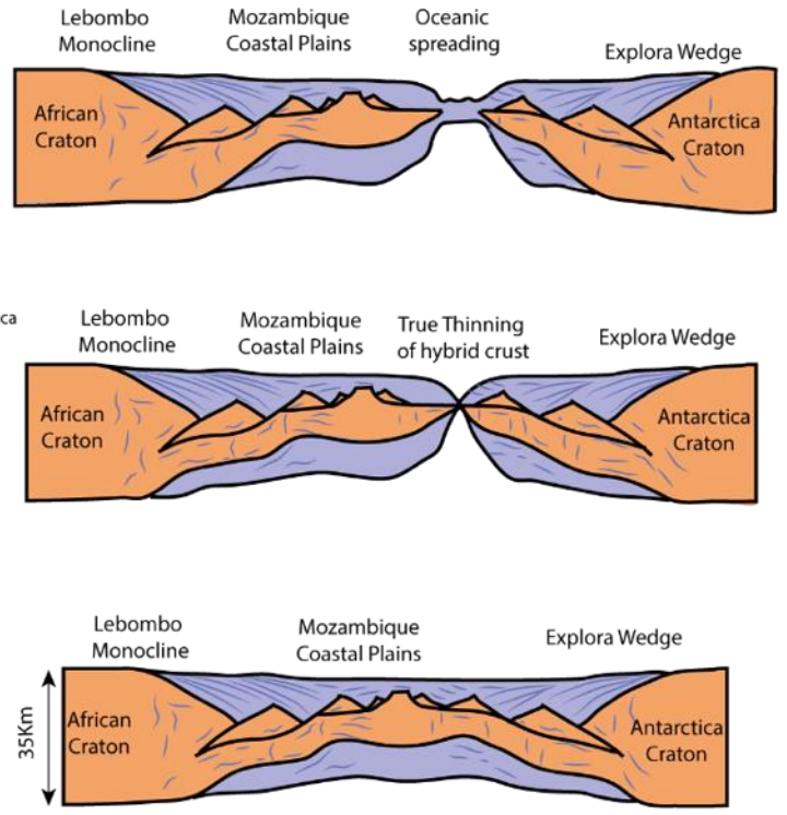
Figure 28: Schematic evolution of the Mozambique-Antarctica magma-rich extensive system. (0) Tomography picture is shown here for a scale indication of a mantle plume after Koptev et al., 2015. (1) Plume is rising, producing melt as the lithosphere is thinned. This magmatic addition maintains crust to a certain thickness balancing the crustal thinning. (2) The magmatic pulse is over, SDRs may develop. (3) Lithospheric breakup occurs and oceanic spreading begins. Maps indicates the associated plate reconstruction. Crustal scale interpretations are inspired from Foulger et al., 2019.
