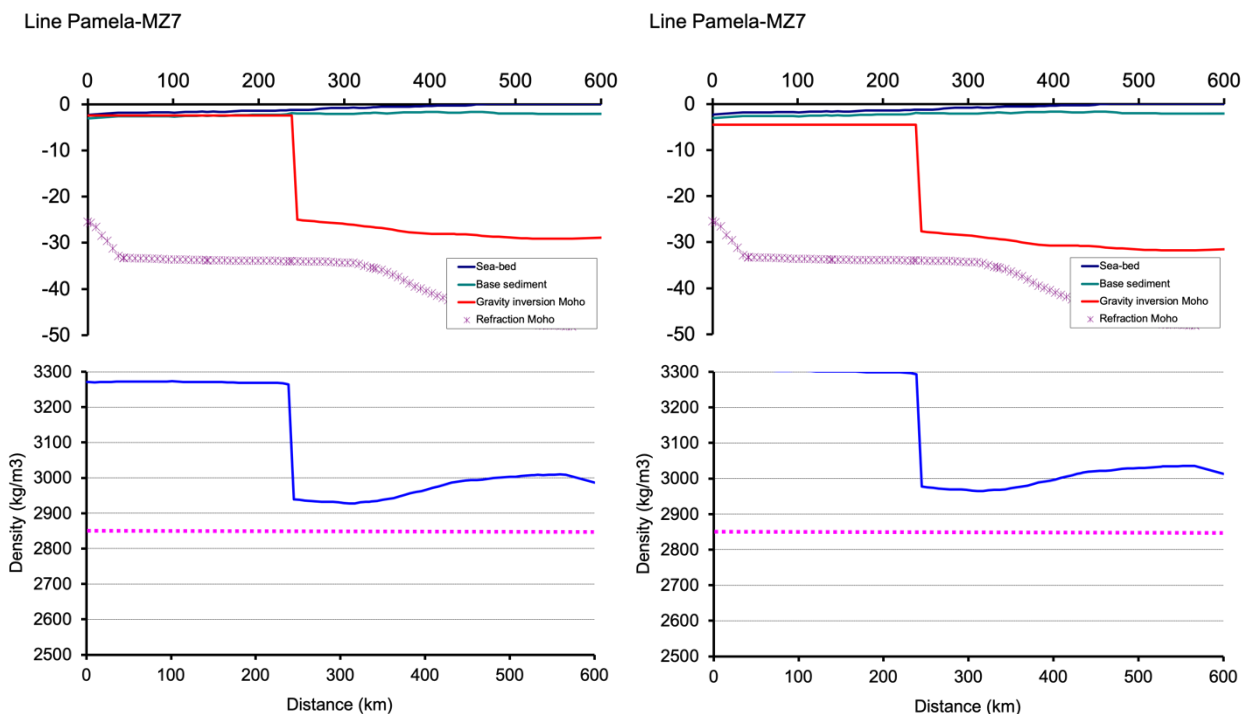
Figure 51: Gravity inversion results using the Total sediment thickness. The column on the left shows the results for the model running a 35km Reference Moho Depth (RMD). The column on the right shows the results running a 32.5km RMD. For each joint inversion, we show the crustal densities need in order to fit the gravity Moho with the Moho interface from the refraction line.
