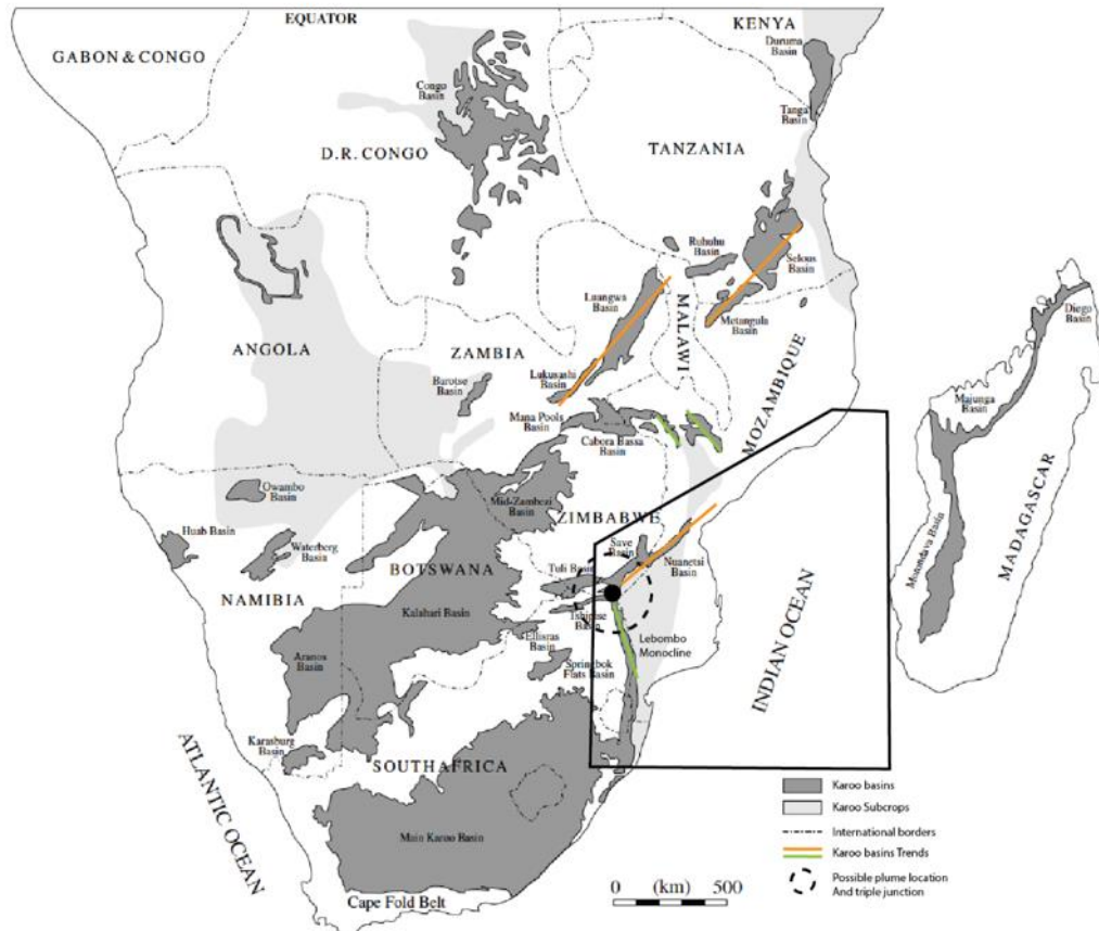
Figure 17: Karoo and Cenozoic rift depressions in southern East Africa. Notice the main NE-SW and NNW-SSE orientations of the rift (after Catuneanu et al., 2005; Johnson et al., 1996; Wescott and Diggins, 1998; Nyambe, 1999; Wopfner, 2002). Position of the triple junction and possible plume location is shown by black circles. Studied area is shown by black polygons.
