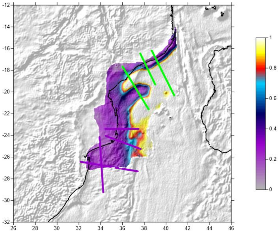
Figure 46: Thinning factor map ( 1-1/\beta ).
