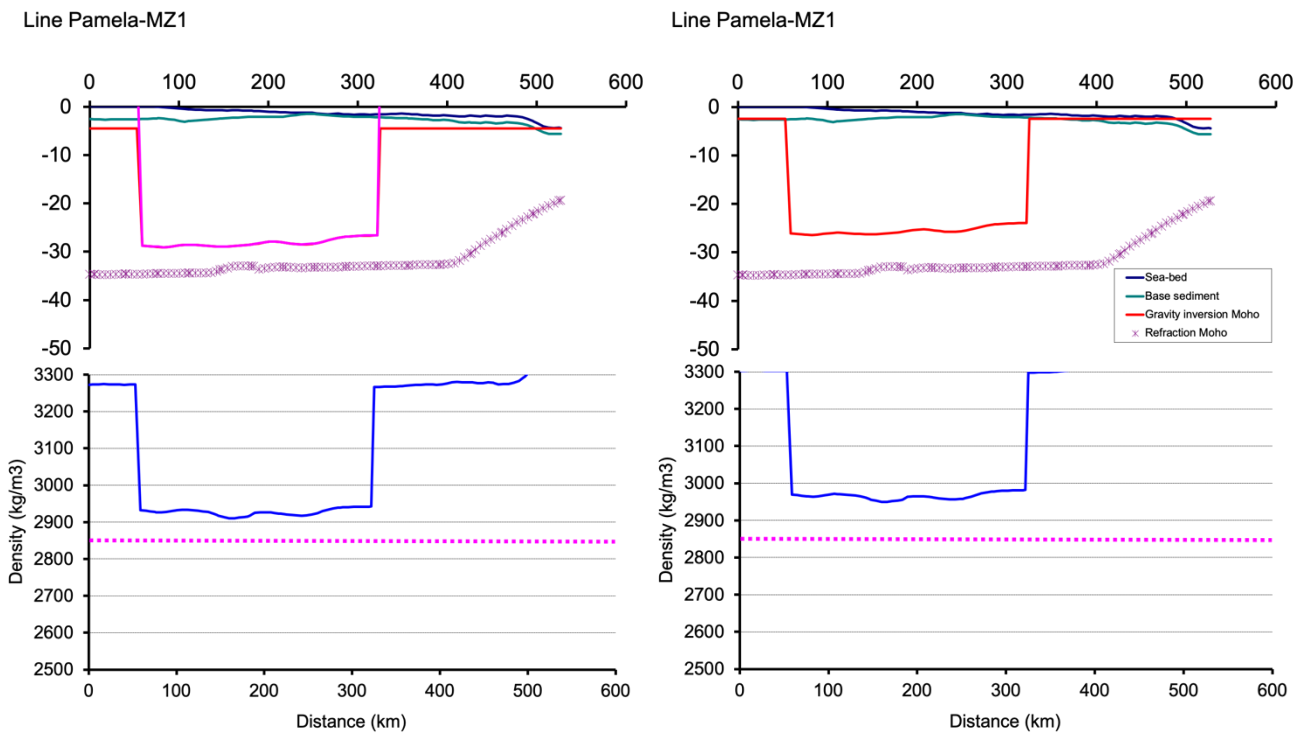
Figure 52: Gravity inversion results using the Total sediment thickness. The column on the left shows the results for the model running a 35km Reference Moho Depth (RMD). The column on the right shows the results running a 32.5km RMD. For each joint inversion, we show the crustal densities need in order to fit the gravity Moho with the Moho interface from the refraction line.
