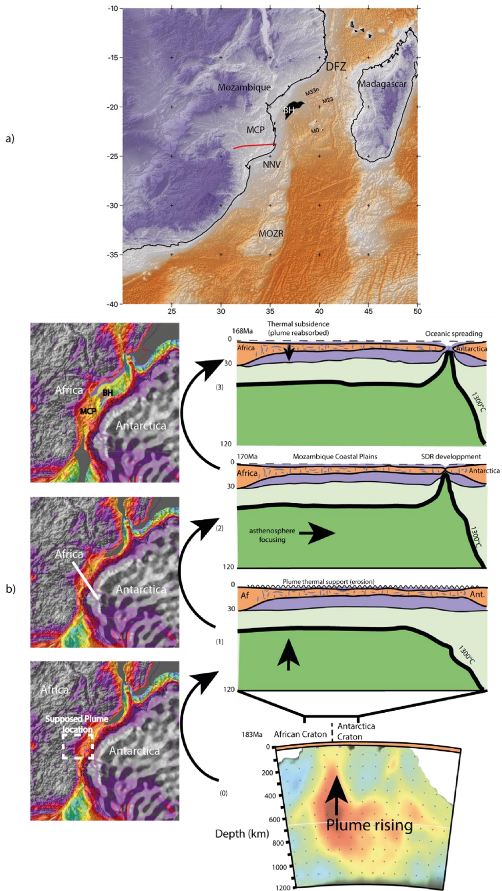
Figure 30: a) Bathymetry of the Mozambique Channel showing the main features and regions analyze in this study. b) Evolution of the Mozambique Coastal Plains associated to the Karoo/Bouvet Plume showing the formation of hybrid crust by the high proportion of magmatic addition.
