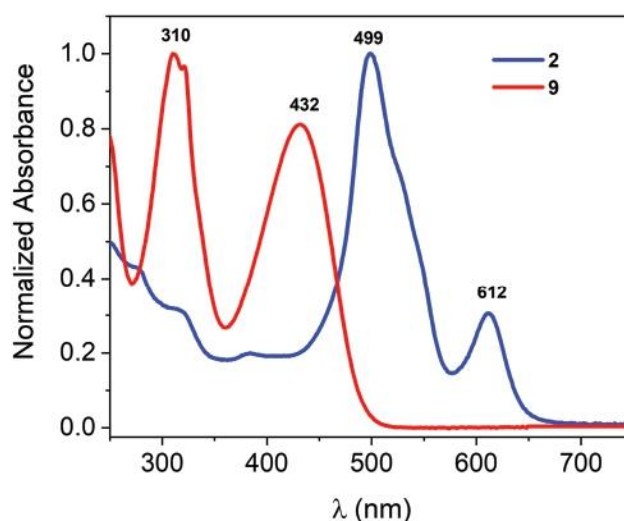
Fig. 1 Absorption spectra of the carbo -benzene 2 and parent molecule 9 in chloroform solution. Absorption coefficients: ε 1 ( 2 , 499 nm) = 5.79 × 10 4 L mol -1 cm -1 at λ = 499 nm, ε 2 ( 2 , 612 nm) = 1.75 × 10 4 L mol -1 cm -1 , ε( 9 , 432 nm) = 1.17 × 10 4 L mol -1 cm -1 .
