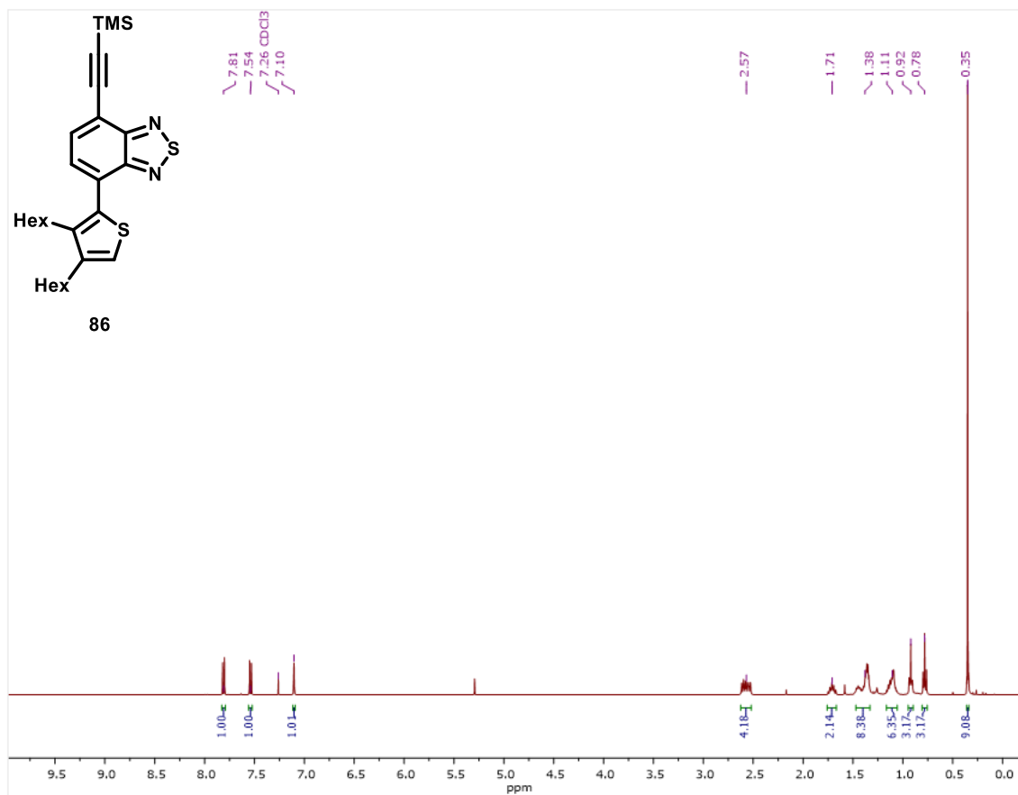
RMN 1 H (400.16 MHz, CDCl 3 ) para 86
