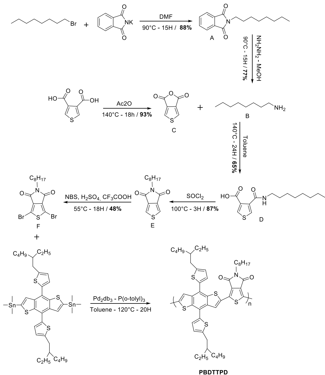
Scheme 1: PBDDTPD synthesis
