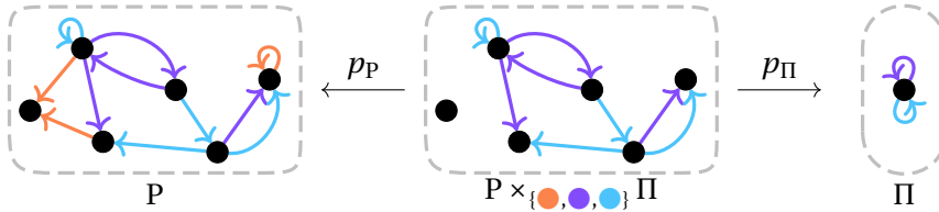
Figure 4.13: Deletion of all the \bullet -arcs using a product in \{\bullet, \circ, \triangle\} - Graph .
