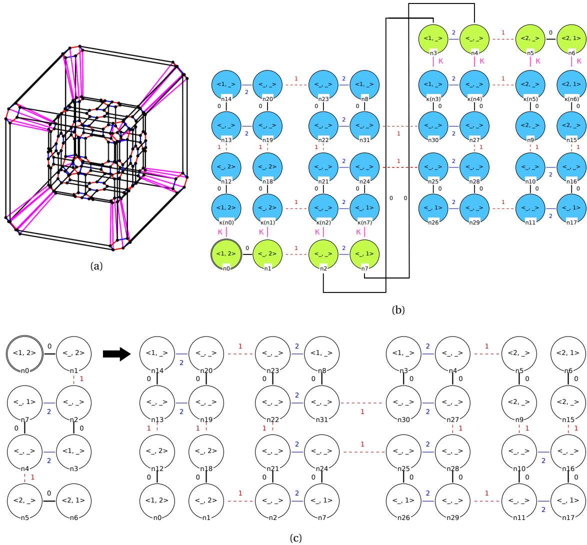
Figure 7.11: Folding the quad subdivision on the joint representation of the cube: (a) the joint representation \kappa(L,R) for quad subdivision of the cube, green nodes belong to the rule's left-hand side and blue nodes to the right-hand side. (b) the joint representation of the rule scheme retrieved by the topological folding algorithm, and (c) the final rule scheme.
