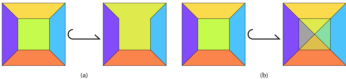
Figure 5.2: Modeling operations with geometric modifications: (a) edge removal, (b) barycentric triangulation.
