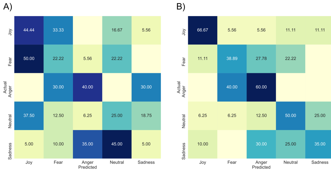
Figure 27 Confusion Matrices for Naive Bayes and SVC on 2 nd Dataset
