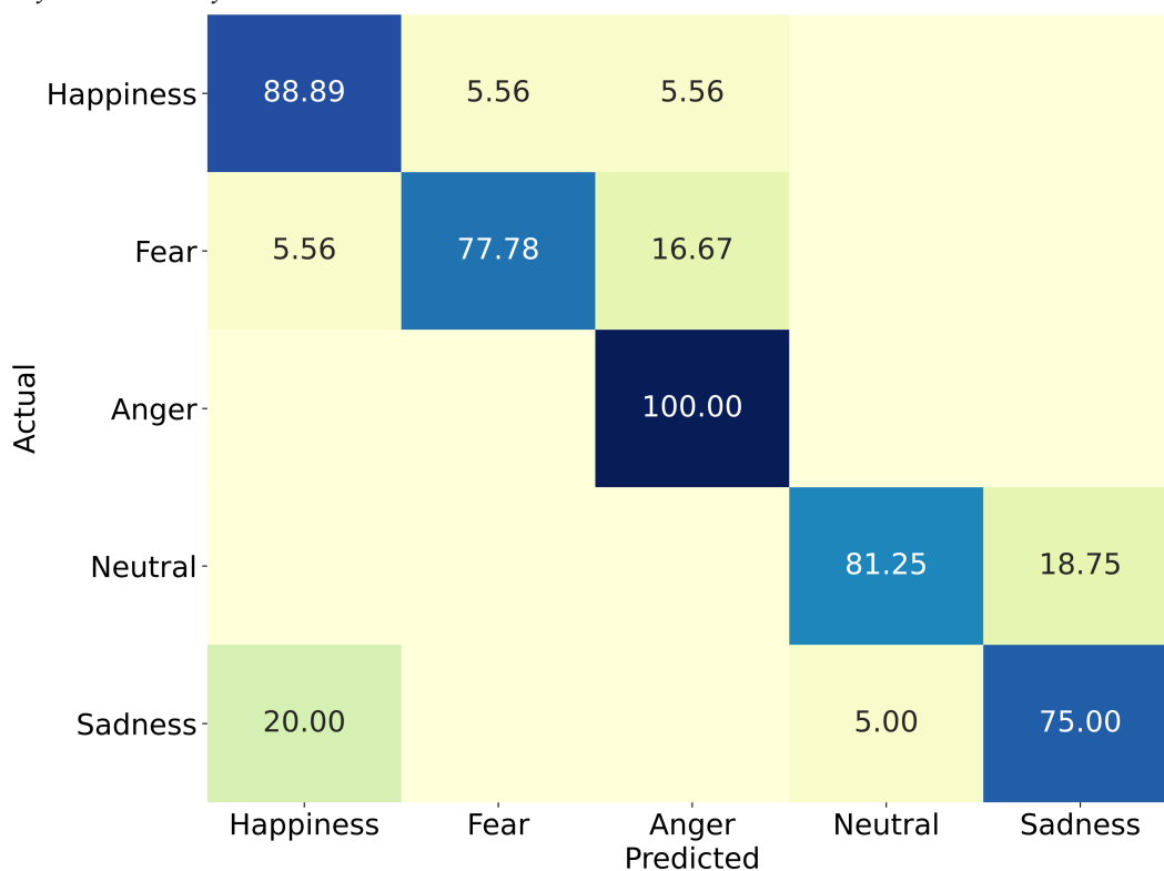
Figure 26 Confusion Matrix for DeeREKt on 2 nd Dataset
