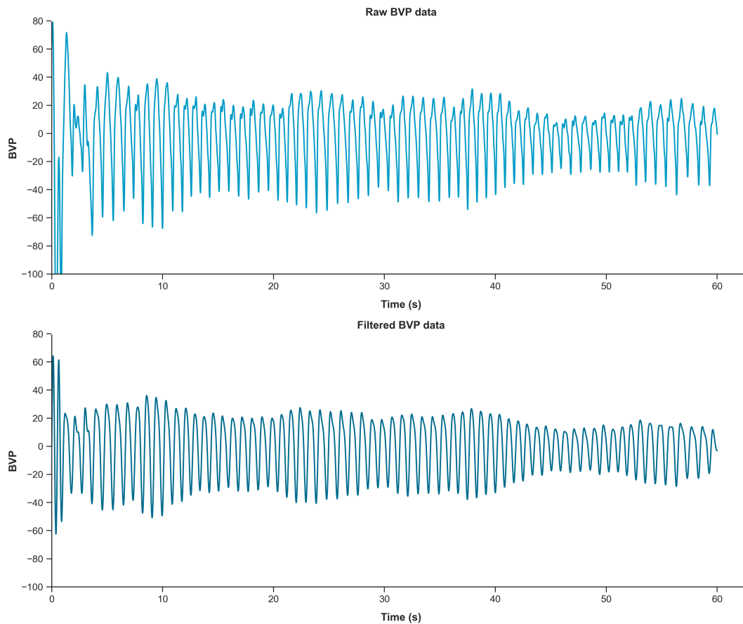
Figure 31 Example of a Raw and Filtered BVP Signal
