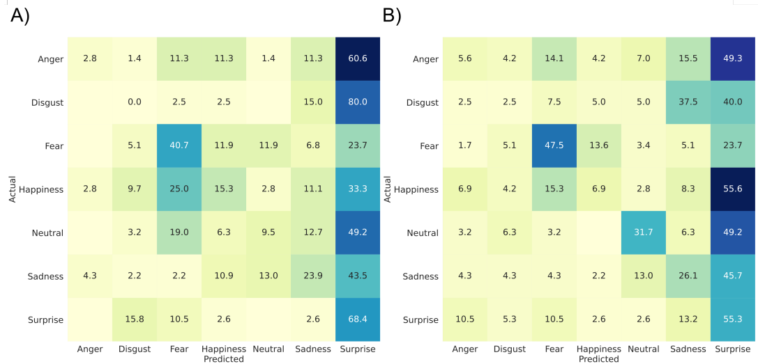
Figure 24 Confusion Matrices for Naive Bayes and SVC on the 1 st Dataset
