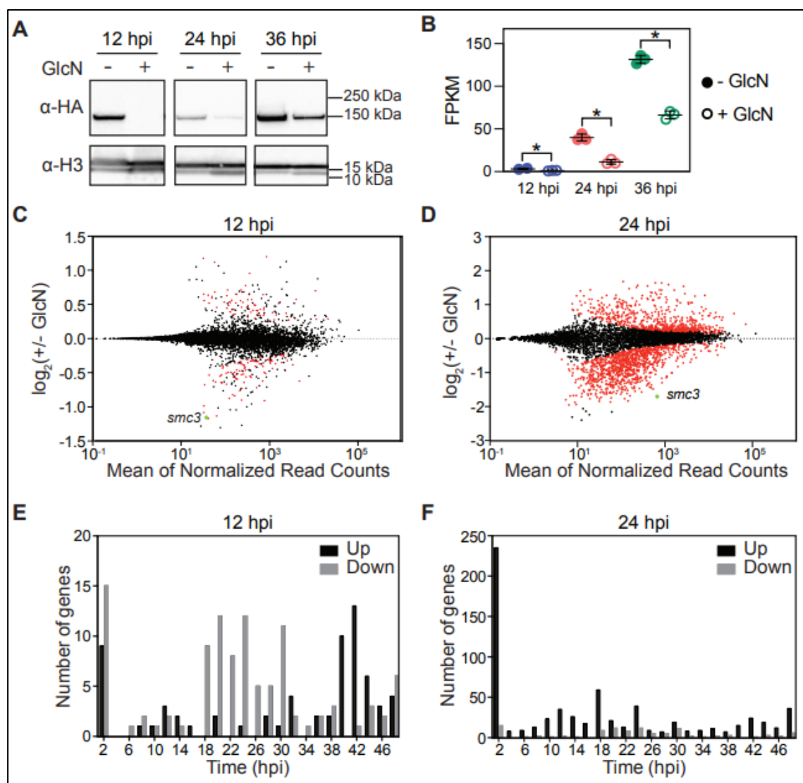
Figure 2.3. SMC3 inducible knockdown results in deregulation of genes in P. falciparum . (A) Western blot analysis of nuclear extracts at 12, 24 hpi and 36 hpi from a clonal population of SMC3-3HA- glmS parasites in the absence (-) or presence (+) of glucosamine (GlcN). SMC3-3HA is detected with an anti-HA antibody. An antibody against histone H3 is used as a control for the nuclear extract. Molecular weights are shown to the right. (B) RNA-seq of an SMC3-3HA- glmS clone shows smc3 transcript levels (FPKM) at 12 ( q = 8.5 \times 10^{-3} ), 24 ( q = 1.3 \times 10^{-39} ) and 36 hpi ( q = 4.14 \times 10^{-54} ) in the absence (circles) or presence (squares) of glucosamine (GlcN). P-values are calculated with a Wald test for significance of coefficients in a negative binomial generalized linear model as implemented in DESeq2 (Love et al., 2014). q = Bonferroni corrected P-value. Corresponding data can be found in Tables 6 and 7. (C) and (D) MA plots of \log_2(\text{glucosamine-treated/untreated}, M) plotted over the mean abundance of each gene (A) at 12 hpi (C) and 24 hpi (D). Transcripts that were significantly higher (above x-axis) or lower (below x-axis) in abundance in the presence of glucosamine are highlighted in red ( q \leq 0.1 ). smc3 is highlighted in green. Three replicates were used for untreated and glucosamine-treated parasites, with the exception of the untreated 12 hpi parasites, for which there were two replicates. P-values were calculated with a Wald test for significance of coefficients in a negative binomial generalized linear model as implemented in DESeq2 (Love et al., 2014). q = Bonferroni
