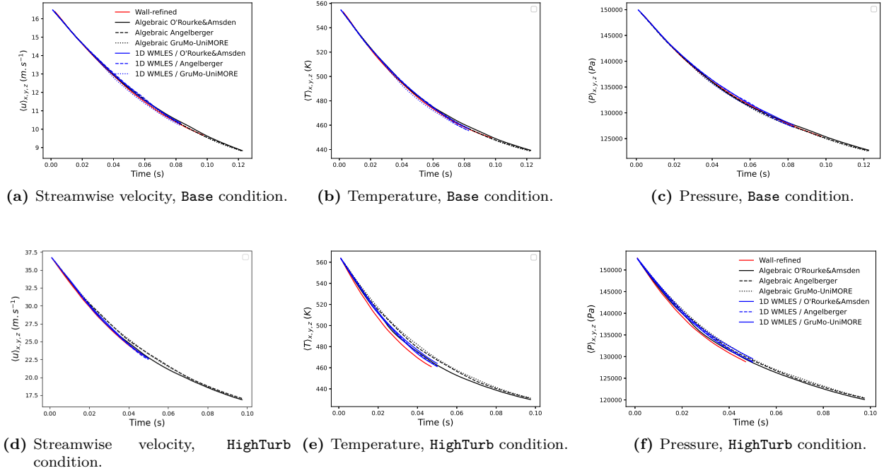
Figure 6.6: Evolution of the volumetric average of streamwise velocity, temperature and pressure over the domain for the Base and HighTurb conditions: Algebraic and ODEs based WMLES.
