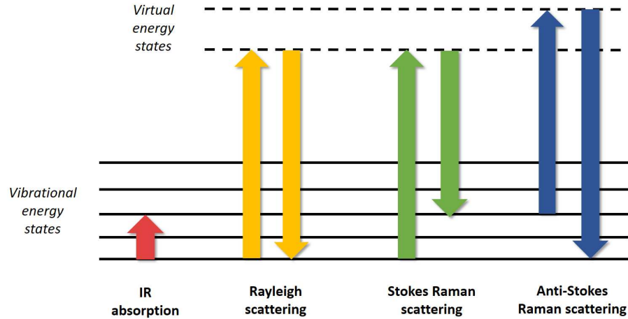
Figure 2.10: IR, Rayleigh and the Stokes and anti-Stokes Raman scattering, with the phonon picture. Resonance are described by a ground state and an excited state. Virtual intermediate states are represented with dotted lines.
