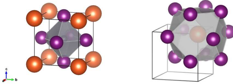
Figure 1.8: Perovskite structure representation: octahedral representation (left) and cuboctahedral representation (right). ABX_3 : A in orange, B in grey and X in purple. Extracted from [25]
