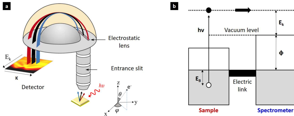
Figure 5.3: (a) Schematic view of a hemispherical electron analyzer, adapted from [214]. (b) Energy relation between sample and analyzer.
