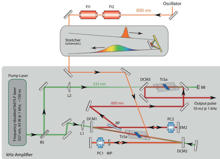
Figure 4.3: Sketch of the regenerative amplifier (RegA) and single pass amplifier (SPA). Oscillator seeds first go through two Faraday isolators (FI1 and FI2) preventing back reflections. Then, they are stretched by a grating stretcher before entering the RegA. A waveplate (WP) and the switching of the Pockels Cell (PC1) allows the seed pulses propagation through the first Ti:Sapphire crystal (Ti:Sa). Ti:Sa is pumped by a 527 nm pump LASER, which is recycled between the two dichroic mirror (DCM1 and DCM2). The polarization of the generated 800 nm pulses rotate after switching the second Pockels cell (PC2) and are further amplified in the a second Ti:Sapphire crystal (Ti:Sa). Extracted from [75].
