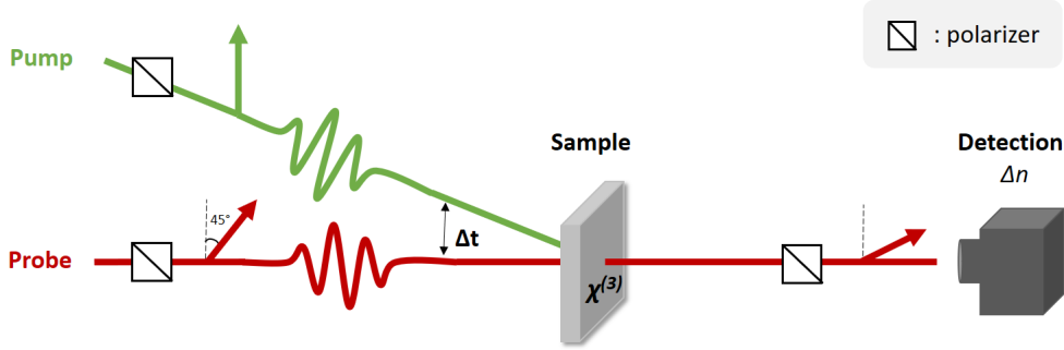
Figure 4.1: Basic sketch representing OKE experiment. Probe pulse (red) is polarized at 45° with respect to the excitation pump pulse (green). The birefringence \Delta n induced in the sample is measured by the change of polarization of the probe by the detection system. \chi^{(3)} is the third-order electric susceptibility of the sample, connecting the different electric fields involved in the FWHM process.
