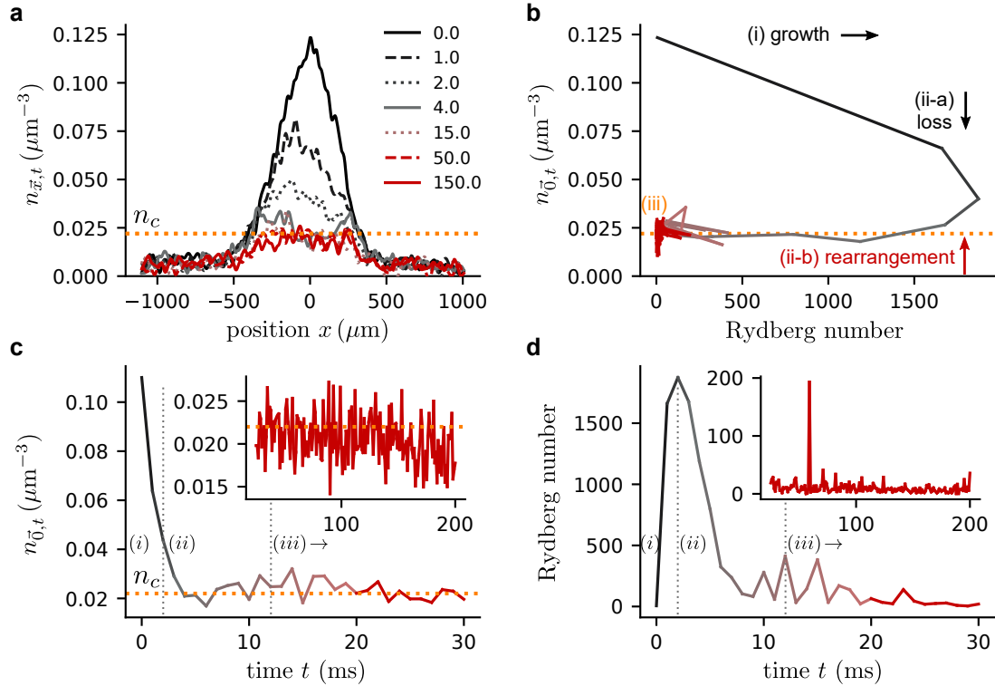
Fig. 4.7: Evolution of the spatial density profile during SOC dynamics in the dipole trap. a Atom density n_{\vec{x},t} cross section through the center of the cloud after Rydberg laser exposure times of 0, 1, 2, 4, 15, 50 and 150 ms (see labels). Initially at t = 0 ms (black line), we observe an approximately Gaussian density profile as expected for the thermal cloud in the dipole trap. Fast loss in the center of the cloud results in a dip after t = 4 ms (gray line). For later times, the density profile shows a flat top at the critical density n_c (orange dotted line) while at the same time the width of the cloud reduces. The three-dimensional density was reconstructed using an inverse Abel transformation on absorption images (see text for more details). b Atom density in the center of the cloud against the corresponding cloud-integrated Rydberg excitation number during the SOC dynamics up to 200 ms. Initially, we start with a density n_{0,t} \approx 0.125 \mu\text{m}^{-3} and zero Rydberg excitations. Subsequently, we observe a growth of the Rydberg number (i) which comes with a reduction in the atom density (ii-a). Around the critical density n_c , we observe overshoots below as well as above due to the rearrangement of atoms in the trapping potential (ii-b). This mechanism sustains the system close to the critical point (iii) for extended periods. c Central atom density as a function of the laser excitation time t . After a fast initial loss, within the first 5 ms, down towards the critical density, we observe an increase in the density due to refilling in the range 10 – 20 ms, before it drops back down again after around 30 ms. At later times, the atom density stays quite constant around n_c from 25 up to 200 ms (see inset with same axes dimensions). d Corresponding number of Rydberg excitations in the atom cloud as a function of the laser excitation time t . The excitation number quickly rises within the first 2 ms before it drops due to the simultaneous reduction in the atom density. This is followed by a range of larger activity fluctuations (10 – 20 ms) which we attribute to fast refilling of atoms. At later times from 25 – 200 ms, the activity is small, but generally non-zero with fluctuations to higher numbers (see inset with same axes dimensions). Note that each time point corresponds to an individual run of the experiment.
