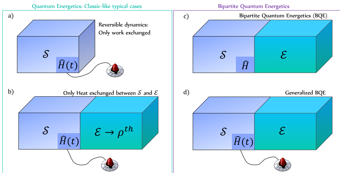
Figure 2.1: Typical classical-like situations in which a quantum system interacts with a classical environment are depicted in the left box. a) When a quantum system is closed that its Hamiltonian is monitored by external classical drive its evolution is unitary and it only exchanges work with its environment. b) When this system is in contact with a bath the energy exchanged with it is only in the form of heat. The bipartite quantum energetics formalism allows to characterize the energy exchange between two quantum systems, when the total Hamiltonian is time independent c) or time-dependent d)
