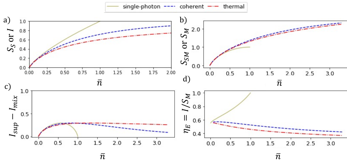
Figure 5.7: Mutual information and entropies of an initially pure qubit state measured by single photon (yellow solid), coherent (blue dashed) and thermal (red dash-dotted) fields. The qubit system entropy or equivalently mutual information I a), meter field entropy or equivalently total entropy b) are plotted as functions of the average number of photon in the fields \bar{n} . The mutual information is compared between the case with and without coherences in the measured system c). The energetic efficiency, as quantified by the ratio between the mutual information and the meter entropy is also presented in d), which only reaches its maximum value for single photon field.
