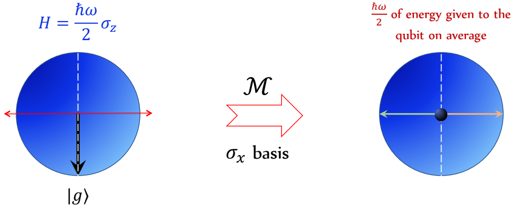
Figure 1.4: Exemple of a projective measurement induced energy exchange. Here by measuring the operator \sigma_x we can provide \hbar\omega/2 of energy on average to the system given that it was initially in the ground state (black arrow) of its Hamiltonian \frac{\hbar\omega}{2}\sigma_z . The final state of the unread measurement is represented by the black sphere and the ones conditioned on obtaining a value +1 (in red) or -1 (in green) for the average of \sigma_x are arrows on the equatorial plane.
