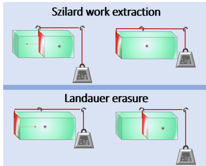
Figure 1.3: Landauer erasure and Szilard work extraction as two opposite mechanisms.
