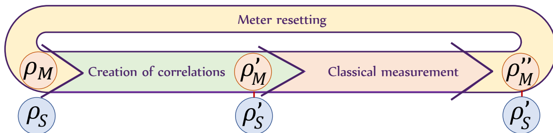
Figure 5.1: The three steps of a cycle of measurement and erasure can in the most general case affect both the system S and meter M 's respective states \rho^S and \rho^M , if the system has coherences in its measurement basis. At the end, only the meter state has to be resetted which implies that the correlations built during the pre-measurement step and represented with a red line are destroyed.
