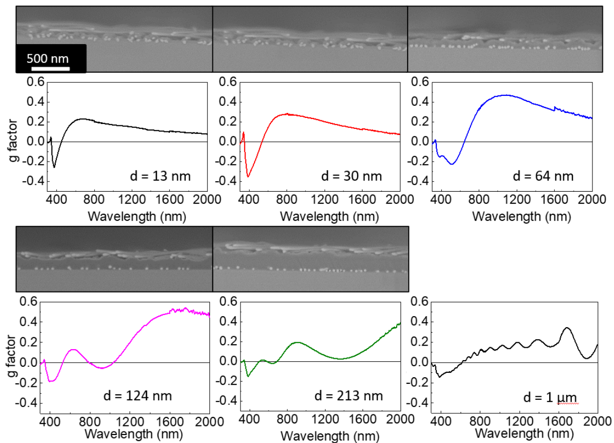
Figure 72. g-factors of samples with different interlayer spacing d and an angle between the AgNW orientation direction fixed at 60° and corresponding cross-section SEM images.
