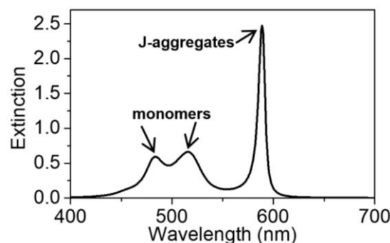
Figure 88. Chemical structure of TDBC and the extinction spectrum of its solution in water at a concentration of 0.1 mg/ml.
