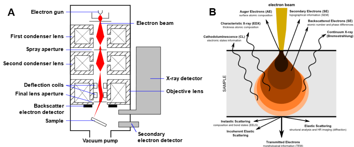
Figure 40. (A) Schematic representation of a SEM. 255 (B) Interaction pear showing the different interactions between the electrons and the sample. 256
