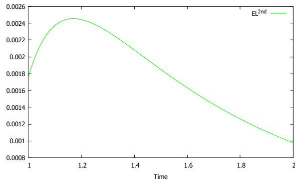
(b) On \mathbb{T}_1 , x_0 = 1, \Delta x_0 = 0.1, h = 0.01
