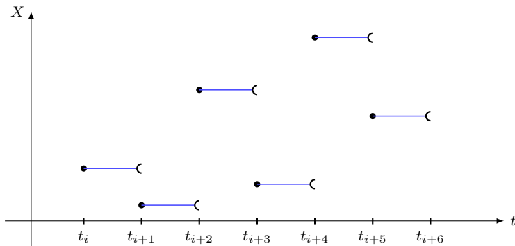
Figure II.2: \mathcal{P}_0^+ -interpolation mapping
