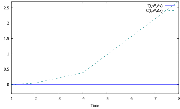
(c) On \mathbb{T}_2 , x_0 = 0, \Delta x_0 = 0.1, n = 3
