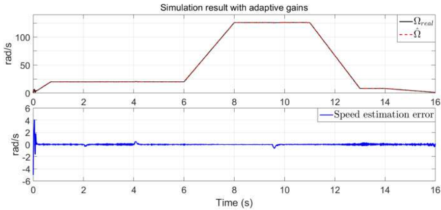
Figure 4.17 – Simulation test: Speed estimation and estimation error
