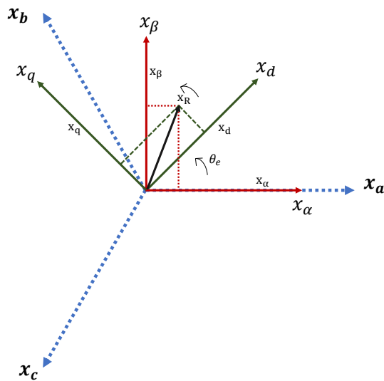
Figure 1.6 – Park transformation
