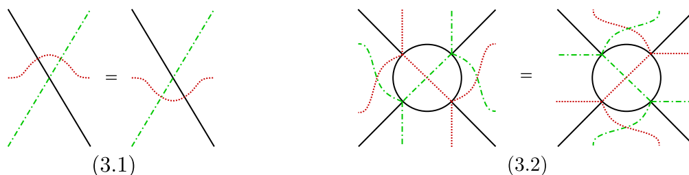
Figure 15.13: Three-color relation
