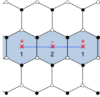
Figure 9.16: A piece of the dimer for a fixed point orientifold realizing the 3 - 2 model with an \text{SO}(N_1 + 1) \times \text{USp}(N_2 + 2) subsector.
