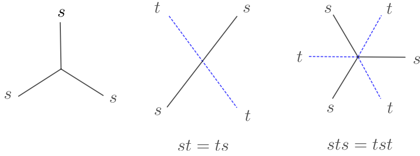
Figure 15.9: Vertex types
