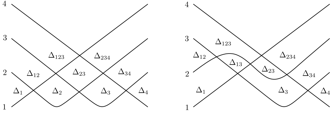
Figure 1.3: Pseudo-line arrangements.
