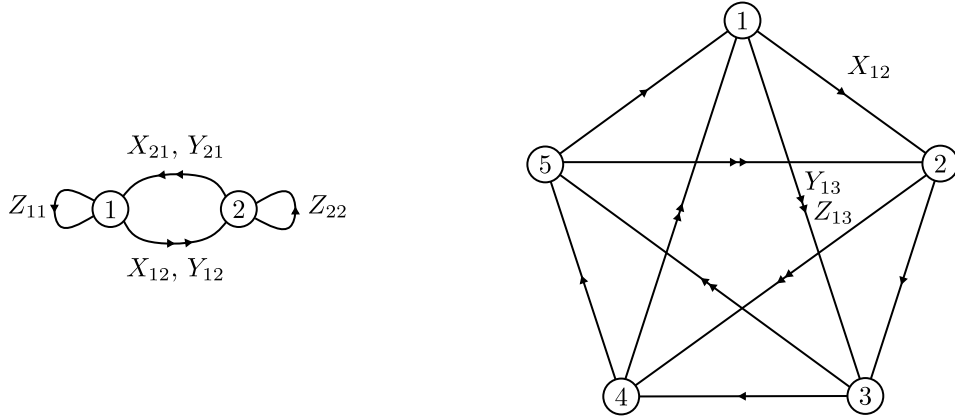
Figure 7.1: The quivers corresponding to D3 branes at \mathbb{C}^2/\mathbb{Z}_2 \times \mathbb{C} (left) and \mathbb{C}^3/\mathbb{Z}_5 (right).
