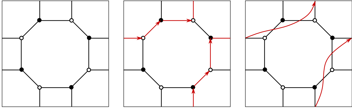
Figure 10.1: A dimer model, a zig-zag path and a zig-zag strand.
