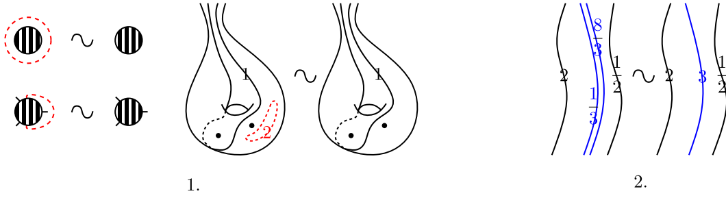
Figure 3.15: Equivalence relations for rational \mathcal{X} -laminations.
