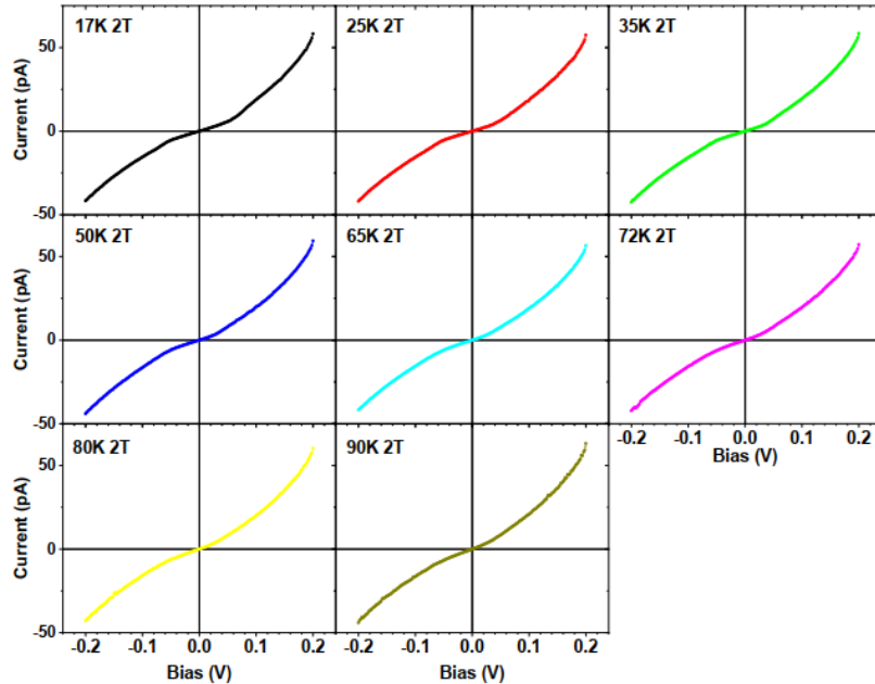
Figure 7.3. Spin-flip excitation. I(V) data at H=+2T for various temperature points (T) acquired for the nanopillar of size 500nm crafted from Si|SiOx|Cr(5)|Fe(50)|CoPc(20)|Co(10)|Cr(5) stack.[33]
