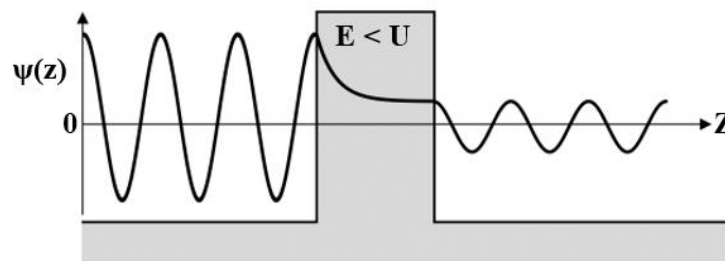
Figure 1.1. Schematic representation of quantum tunneling at the barrier. The tunneling event takes place only when: i) the incoming particle exhibits quantum properties (wave-particle duality), and ii) the energy ( E = \hbar\omega ) of which is less than the barrier height ( U ), i.e. E < U . Along the propagation axis- z , at any point the amplitude of the wave associated with the quantum particle is given by \psi(z) = \exp(ik \cdot z) , where \psi is the wavefunction and k is the wave-vector along the propagation axis- z .
