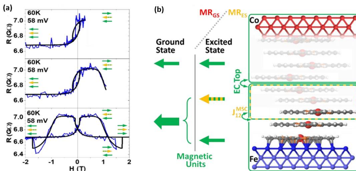
Figure 7.5. Spin-flip magnetoresistance. (a) Magnetotransport measurement performed at T=60K and V=58mV reveal three resistance switching due to the magnetization reversal of three magnetic units (green and green/yellow arrows). (b) Schematic of the magnetic units contributing to MR_{GS} and MR_{ES} . In the ground state the CoPc molecular spin chain forms a relatively harder unit together with the Fe|CoPc spinterface and the underneath bottom Fe electrode (represented by the bottom large green box that also contains green/yellow box), however, in its spin-flipped excited state, the CoPc molecular spin chain acts as a distinct magnetic unit (represented by green/yellow box and arrow) with a coercive field and contributes only to MR_{ES} . The junction's imperfectly controlled portion appears semi-transparent. The macrospin model's coupling terms ECTop and J_{12}^{MSC} between the central and top/bottom units are shown. See the texts for more detail. The fit (shown by black line in panel (a)) was performed using the parameters K_t/M_t = 0.26T , \theta_{Mt} = 60^\circ , K_b/M_b = 4.95T , \theta_{Mb} = -4^\circ , ECTop = -0.05T , J_{12}^{MSC} = 1.28T , R_0 = 6.68G\Omega , MR_{GS} = -2.4\% and MR_{ES} = 5.1\% . [33]
