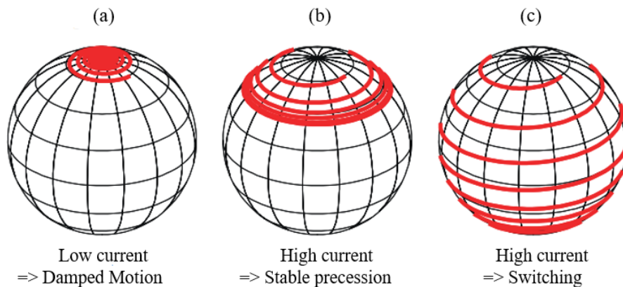
Figure 1.20. Schematic representation of three possible scenarios during STT event: (a) low current leading to the damped motion, (b) high current leading to stable and steady magnetic precession, and (c) High current leading to switching free layer magnetization in MTJs. The figures are taken from ref [11].
