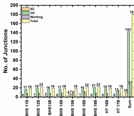
Figure 6.17. The success rate of ‘microfluidic pen lithography’ technique. Graphical representation of the prober results for the nanopillars fabricated from a series of capped hybrid trilayer stacks. The X-axis represents the beads processed capped hybrid sample, while the Y-axis shows the frequency of short-circuited (pink), open-circuited (green), working (purple) and total (yellow) nanopillars fabricated from different capped trilayer hybrid stacks.
