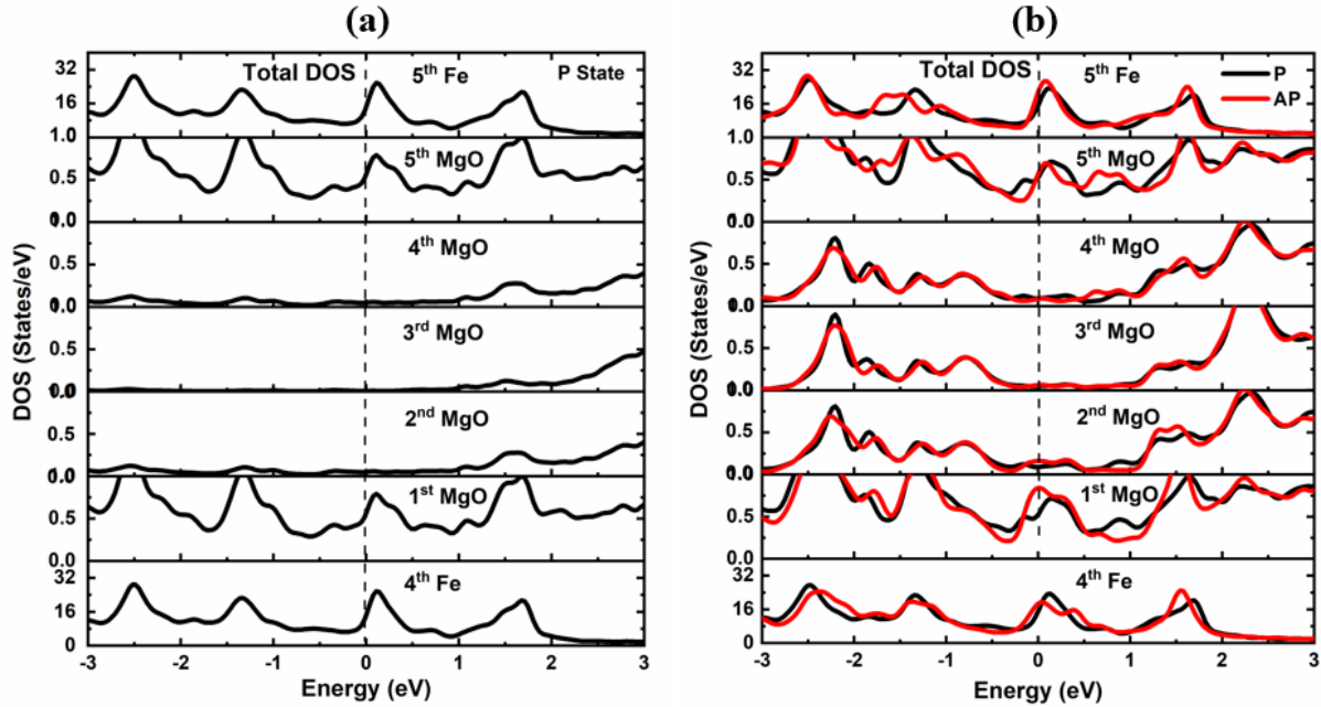
Figure 4.19. Total density of state (DOS) calculated for the Fe(1-4ML)|MgO(5ML)|Fe(5-7ML) MTJ, with (a) intrinsic/defect-free MgO, and (b) zig-zag F- oxygen vacancy chain within the MgO layer. The bottom 4 th Fe monolayer is for the left electrode and the topmost 5 th Fe monolayer is for the right-side electrode. The black curve denotes the P state whereas the red curve denotes the AP state. The available d-electrons near the E_F from both sides of the FM electrode can be seen contributing to the metallicity up to the 2 nd successive monolayer of MgO tunneling barrier from the interface.
