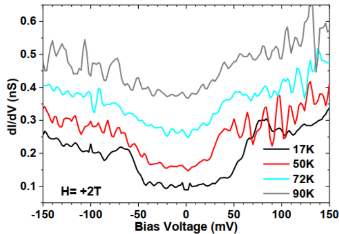
Figure 7.4. Spin-flip excitation. Differential conductance or dI/dV(V) data at H=2T for various temperature points (T) acquired for the nanopillar of size 500nm crafted from Si|SiOx|Cr(5)|Fe(50)|CoPc(20)|Co(10)|Cr(5) stack.[33]
