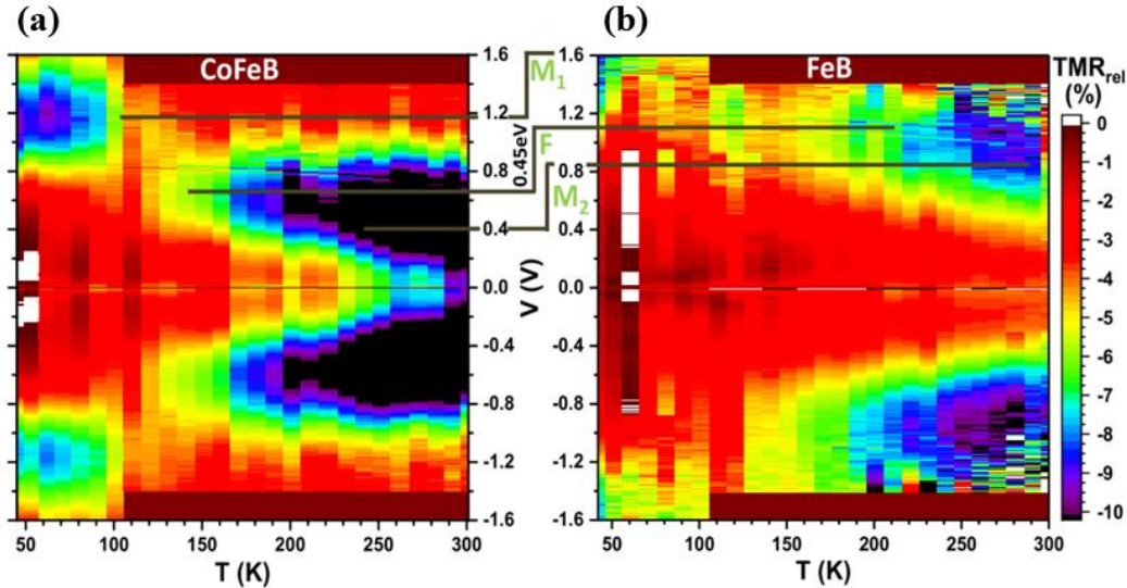
Figure 3.5. TMRrel 3D plots for MTJ devices with the top electrode (a) CoFeB and (b) FeB. The x, y, and z-axis represent the temperature, applied bias, and amplitude of TMR_{rel} respectively. The color scale represents the z-axis or TMR_{rel} amplitude. The shift of the 0.45 eV in the occupied states towards the higher energy values with respect to the Fermi energy is evident when the top FM electrode is replaced from FeCoB to FeB.[119]
