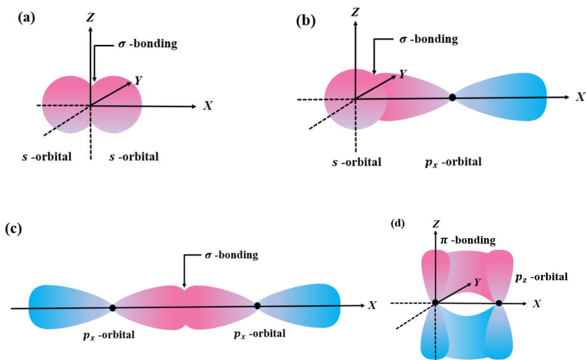
Figure 5.1. Schematic of \sigma - and \pi -bond formation. The \sigma -bond formation due to head-to-head overlap of (a) two s -orbitals, (b) s - and p_x orbital, and (c) two p_x orbitals. The panel (d) shows the lateral overlap of two p_z - orbitals forming the \pi -bond.
