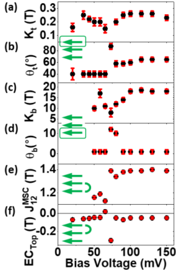
Figure 7.16. Bias dependence of fitting parameters at 17K. Bias dependencies of the strength and angle of the anisotropy field for the (a-b) top and (c-d) central magnetic units. Bias dependencies of the (e) J_{12}^{\text{MSC}} and (f) ECT_{\text{top}} coupling terms. The MR_{\text{ES}} term tracks the dI/dV increase due to spin excitations. At the dI/dV peak, coupling between the MSCs of the top and central unit causes strong changes to their anisotropy parameters (panels h-k) and to the coupling parameters (panels l-m), which distorts the R(H) at 73mV (panel b).[33]
