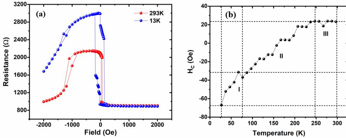
Figure 4.1. A typical magnetotransport performed on MTJ-F device. (a) R(H) plot for MTJ-F device at 13K (blue) and 293K (red). Magnetic state corresponding to 42Oe field remains as P state over the entire temperature range of measurement, (b) Temperature-dependent coercivity ( H_c ) plot.
