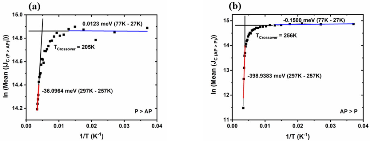
Figure 4.9. Thermal activation energy plots fitted for critical current density ( |J_C| ) for (a) P > AP and (b) AP > P switching, shows how P > AP and AP > P switching scenarios are different from each other.
