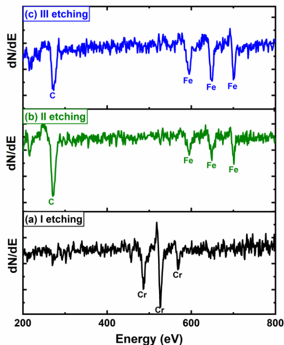
Figure 6.7. 1 st order intensity derivative of Auger signal. after the subsequent etching of inorganic multilayer stack Si|SiO x ||Cr(5)|Fe(50)|C60(2ML)|CoPc(3ML)|C60(5ML)|Fe(10)|Cr(100) with silica beads of 350nm deposited on top surface (capping layer) using the microfluidic pen lithography technique [Section 6.5]. The numbers inside the bracket represent the thickness in nm. For clarity, only the highest intensity peaks are highlighted. The peaks at [272] eV, [489, 529, 571] eV, and [598, 651, 703] eV, and corresponds to C, Cr, and Fe respectively, with the highest intensity peaks at 272 eV, 529 eV, and 651 eV for C, Cr, and Fe respectively.
