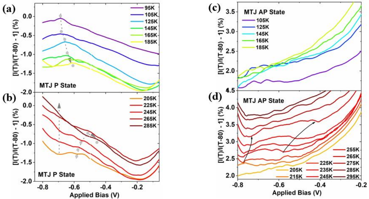
Figure 4.11. I-hat ( \hat{I} -) plots calculated from consecutive high resolution I(V)s performed at \Delta T = T_2 - T_1 = 80K , for (a, b) P state (2000Oe) and (c, d) AP state (-200Oe) for MTJ-F device.
