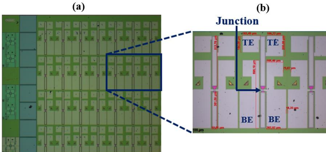
Figure 2.11. Optical image of the MTJ-F nanopillar devices. (a) Microscopic image of the EBL processed multilayer stack taken from an optical microscope, (b) Zoomed image of nanopillar MTJs with two contact pads for both top (TE) and bottom electrodes (BE). In the pink part, the area beneath the metallic contact pad is the nanopillar MTJ device.
