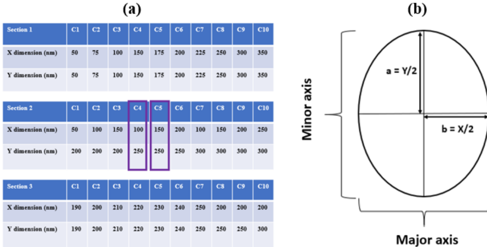
Figure 2.10. Structural details of the MTJ-F nanopillar devices. (a) Dimensions of all the nanopillar devices in nm, (b) dimensions, and geometry of the elliptical devices in section 2 of the processed multilayer stack.
