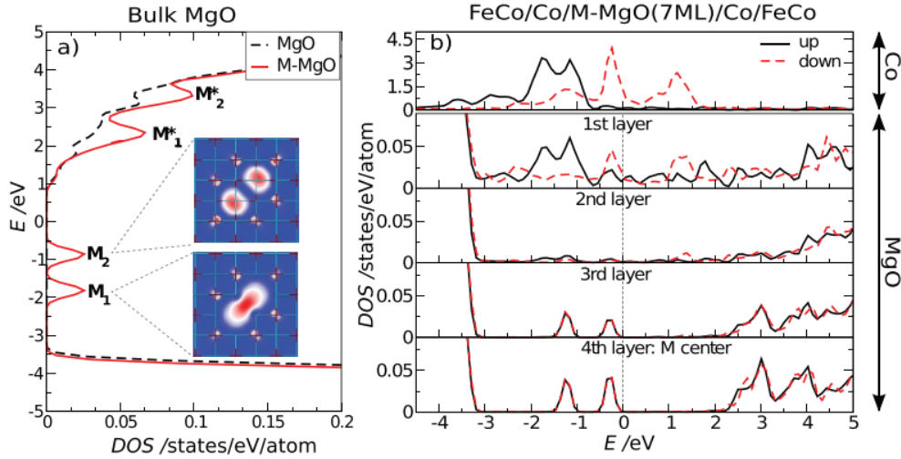
Figure 1.14. Theoretically calculated DOS plots for MgO with and without double oxygen vacancy or M-center. (a) DOS plot (with charge densities in inset) for M-center created within bulk-MgO resulting two localized states M_1 (bonding) and M_2 (antibonding) located at 0.4 eV and 1.1 eV below Fermi energy ( E_F ), (b) Layer-projected, and spin-polarized DOS plots for FeCo|Co|MgO(7ML)|Co|CoFe with M-center at middle monolayer (4 th ) of MgO. The figures are taken from ref [4].
