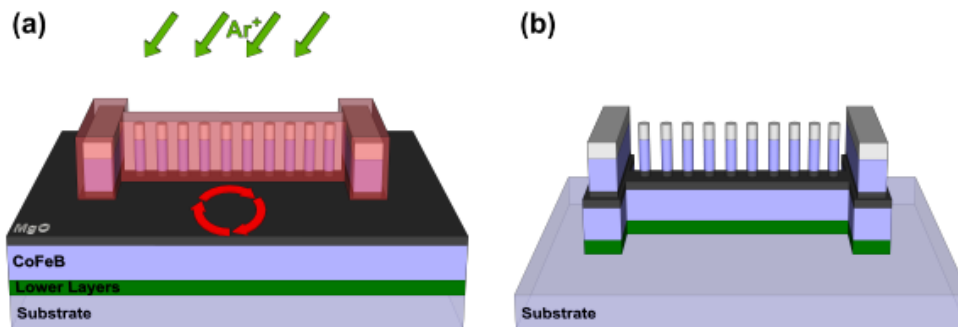
Figure 2.5. Schematics for the photolithography step-II, (a) The step-I pattern is preserved by the developed positive photoresist (pink color) during the Ar ion etching step performed down to the glass (substrate), (b) The pattern created containing bottom electrode and pillars and bottom electrode contact pads after the etching process (a). The figures are taken from ref. [41].
