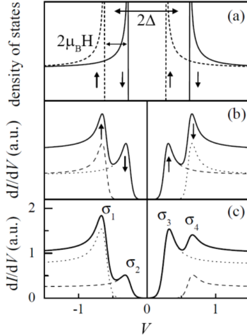
Figure 1.2. Spin dependent tunneling. (a) Zeeman split energy levels ( \pm \mu_B H within the 2\Delta eV energy gap near E_F for superconductor (Al thin film), (b) unpolarized spin tunneling in M|I|S heterostructure with symmetric peaks around E_F , (c) spin-polarized tunneling in FM|I|S heterostructures with asymmetric peaks around E_F . The figures are taken from ref [42].
