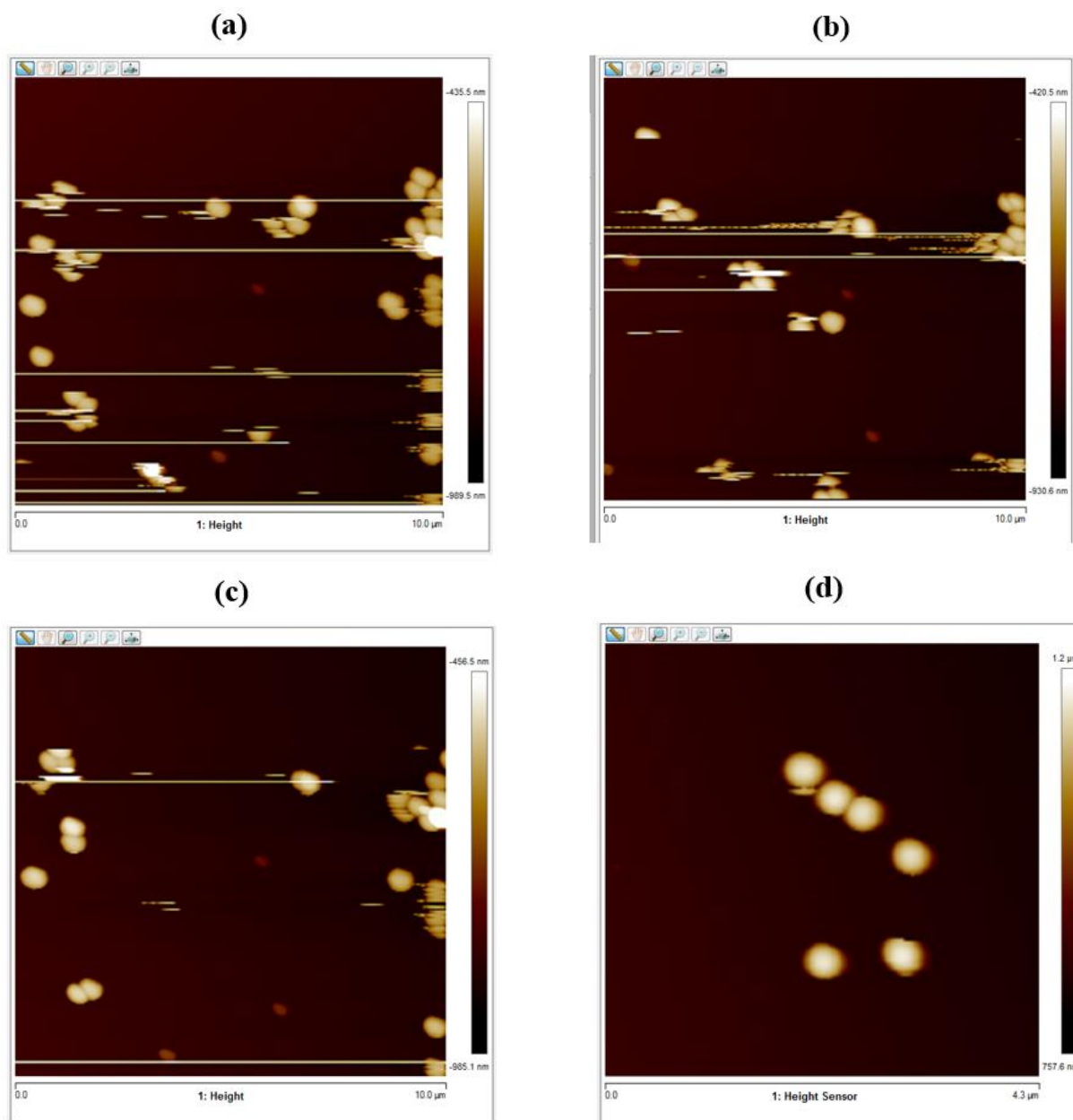
Figure 6.13. AFM images collected on the panel (d) after a series of lateral manipulations performed and on silica nanobeads of \sim 300 nm size loosely bound to the top surface (capping layer) of the capped hybrid trilayer stack shown by the panel (a, b, c),
