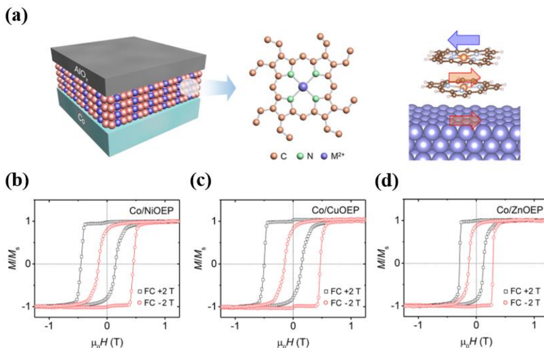
Figure 5.20. Co|MOEP ( M = \text{Ni, Cu, and Zn} ) hybrid bilayer system and the exchange bias. (a) Schematic representation of the Co|MOEP bilayer system and the magnetic coupling. The planar MOEP molecules (shown by blue/red color) are deposited on a Co(111) thin films. Panel (b, c, and d) are the M-H loops showing the molecular exchange bias for the Co(4nm)|MOEP(8nm)| \text{AlO}_x bilayer capped systems with M = \text{Ni, Cu and Zn} respectively. The M-H loops with an open black rectangle (open red circle) correspond to the applied magnetic field of +2\text{T} ( -2\text{T} ) used for the field cooling (FC) procedure. For the M = \text{Ni, Cu, and Zn} systems, the magnitudes of exchange bias H_{\text{EB}} were measured to be -170, -162, and -95\text{mT} , respectively. The figure is taken from ref[170]
