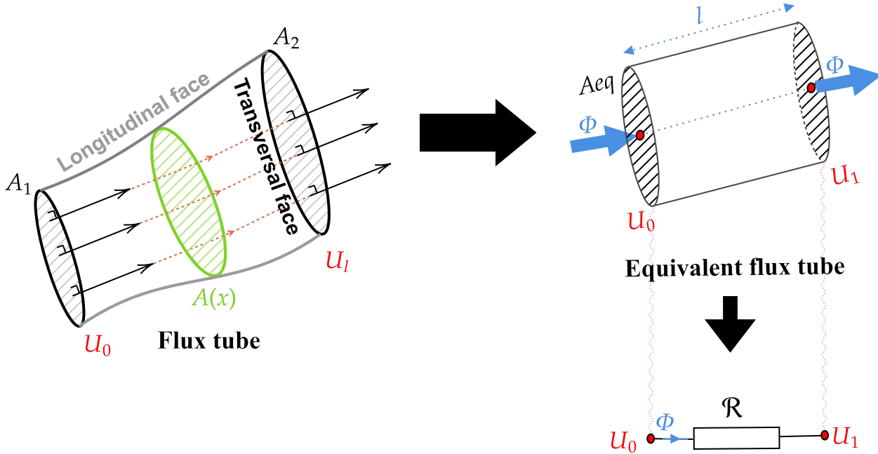
Figure 4.3: Flux tube and its corresponding reluctance
