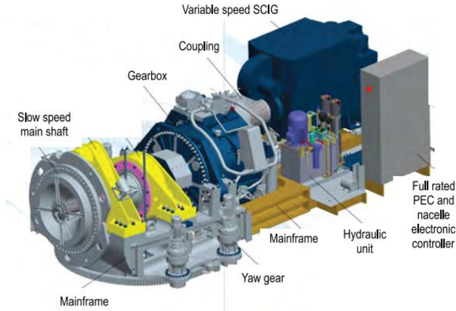
Figure 1.20: Variable-speed full scale converter SCIG-based drive-train driven by gearbox (PS-1800) [6]
