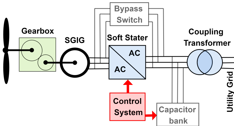
Figure 1.13: The block diagram of a constant-speed wind turbine using SGIG generator
