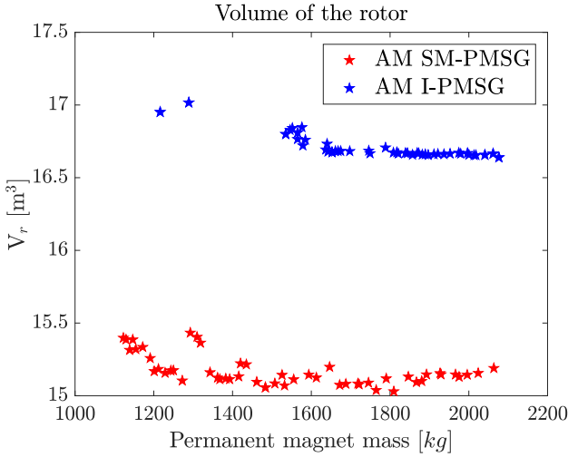
Figure 7.6: Rotor volume of the SM-PMSG
