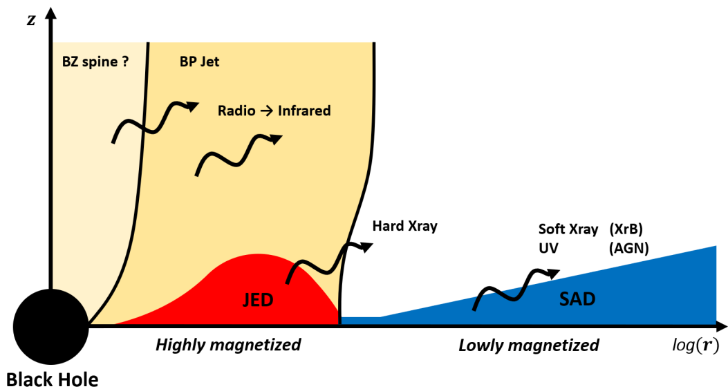
FIGURE 2.1: Schematic view of the section of the inner region of the JED-SAD model. The inner region is highly magnetized and launches a jet, resulting in Jet Emitting Disk. The outer region is lowly magnetized and is a Standard Accretion Disk.
