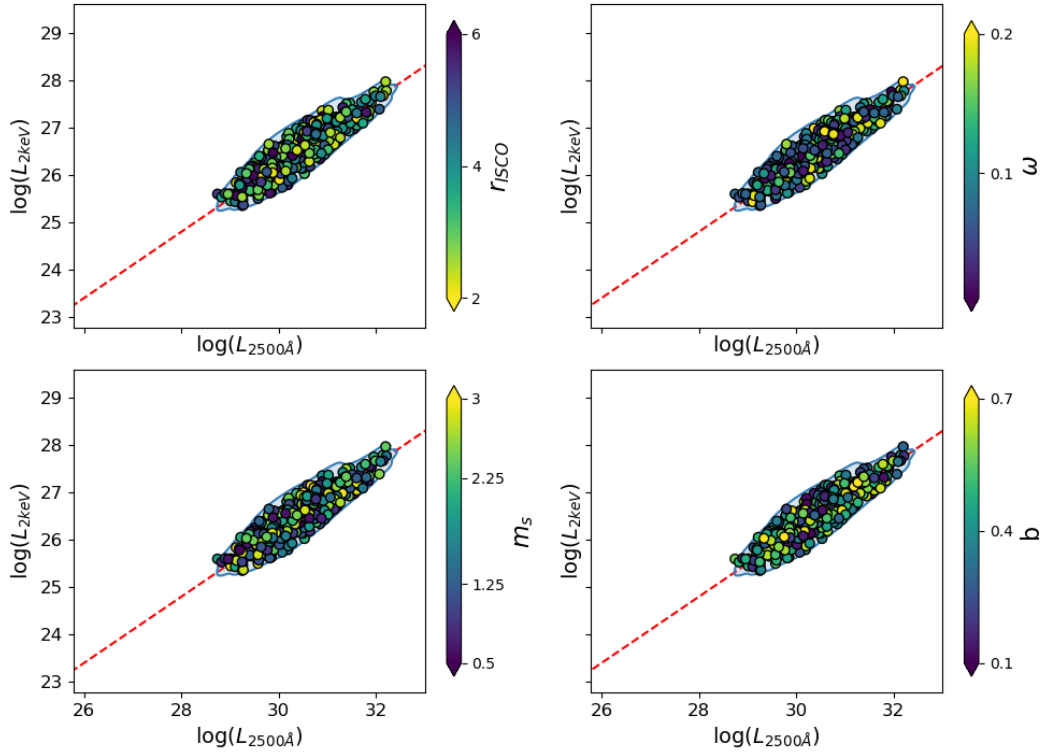
FIGURE 5.20: The simulated sample in the UV–X-ray plane. In the background the L&R sample is plotted in blue. The simulated spectra are colored depending on the value of their JED-SAD parameters: ISCO r_{isco} (upper left), dilution factor \omega (upper right), sonic mach number m_s (bottom left) and power in the jets b (bottom right)
