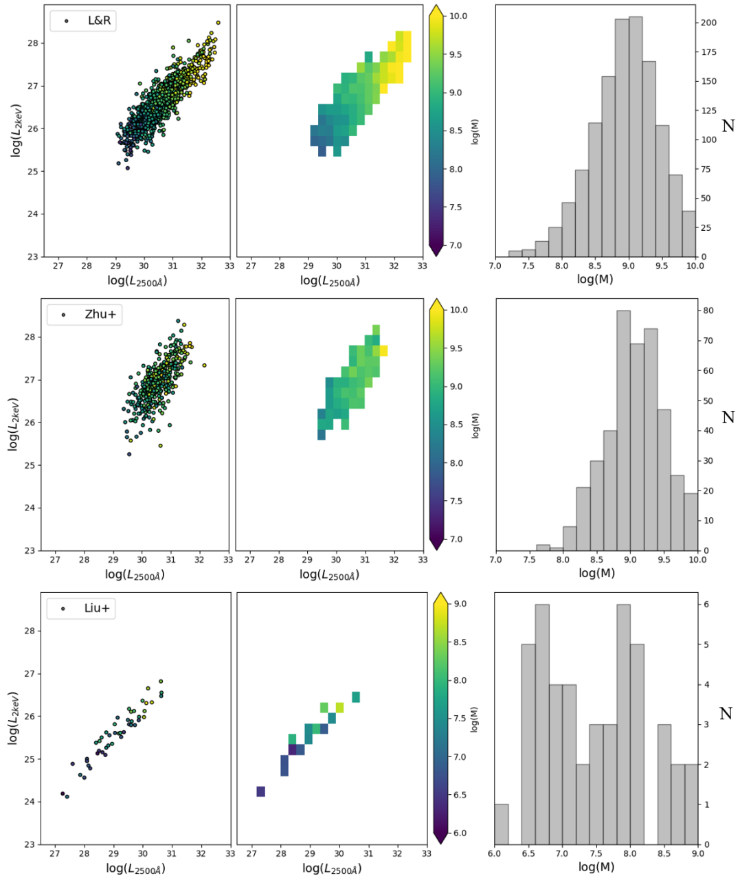
FIGURE 5.5: The black hole masses distribution within the UV–X-ray correlation for the three collected samples. From top to bottom: the L&R sample (Lusso et al. 2020), the Zhu+ sample (Zhu et al. 2020) and the Liu+ sample (Liu et al. 2021). Left: scatter plot of the black hole masses for each sample in the UV–X-ray plane. Middle: Averaged masses along the UV–X-ray correlation for each sample. Both of these panels use the same color scheme. Right: Histogram distribution of the black hole masses for each sample.
