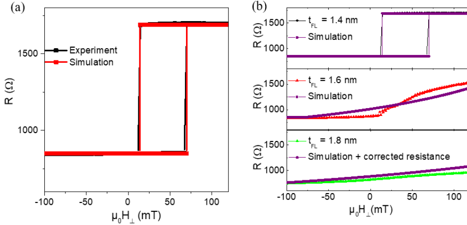
Figure 4.2.3 : (a) Fitting of the out-of-plane magnetoresistance loops of device with free layer thickness of t_{FL} = 1.4 \text{ nm} and a nominal diameter of D_n = 100 \text{ nm} . (b) Using the K_i from fits in (a) to simulate the magneto-resistance loops of t_{FL}=1.6 and 1.8 \text{ nm} using M_s = 10^6 \text{ A/m} , K_i = 8.4e - 4 \text{ J/m}^2 , and \mu_0 H_{int\perp} = 42 \text{ mT} for the out-of plane stray field coming from the uncompensated SAF.
