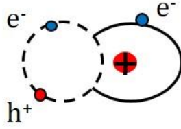
Figure 1.6 Schematic diagram of a donor-bound exciton.
