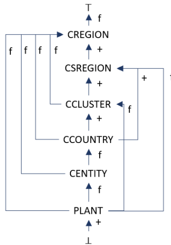
Figure 6.10.: Attribute graph in dimension STORE
