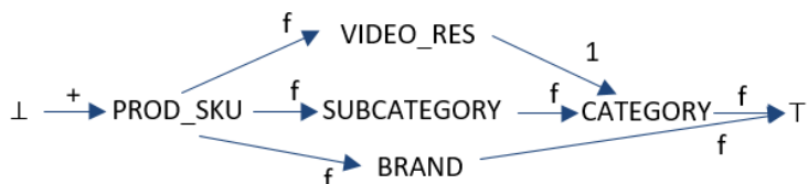
Figure 5.9.: Attribute graph of PROD\_NEW
