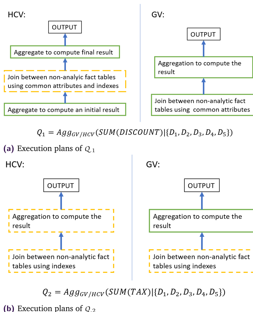
Figure 6.9.: Query execution plans comparisons
