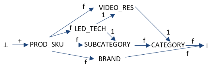
Figure 5.10.: Attribute graph of PROD\_NEW2
