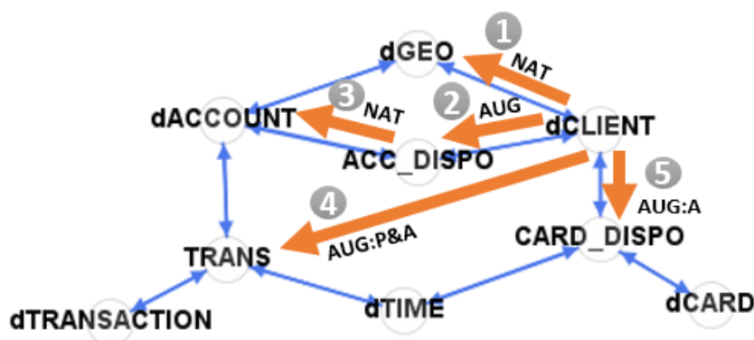
Figure 6.12.: SC graph for the analytic tables
