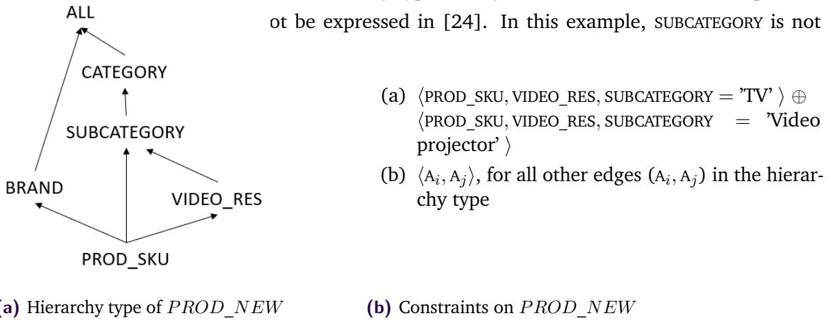
Figure 5.12.: The dimension schema of PROD_NEW
