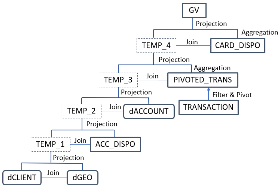
Figure 6.13.: Construction of GV
