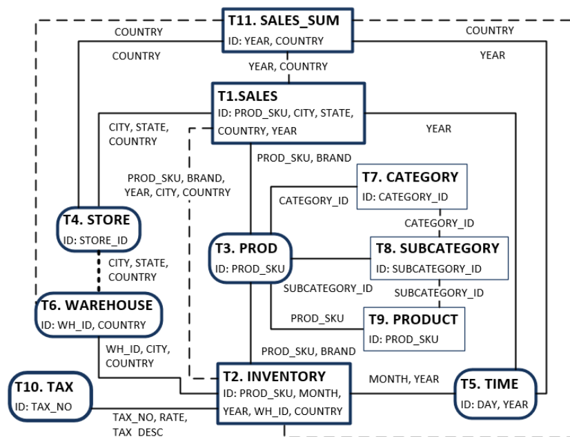
Figure 2.9.: Examples of relationships
