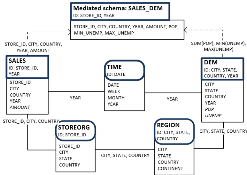
Figure 5.3.: Join relationships and schema matchings
