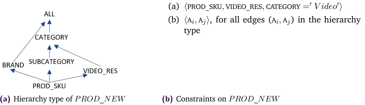
Figure 5.11.: The dimension schema of PROD_NEW
