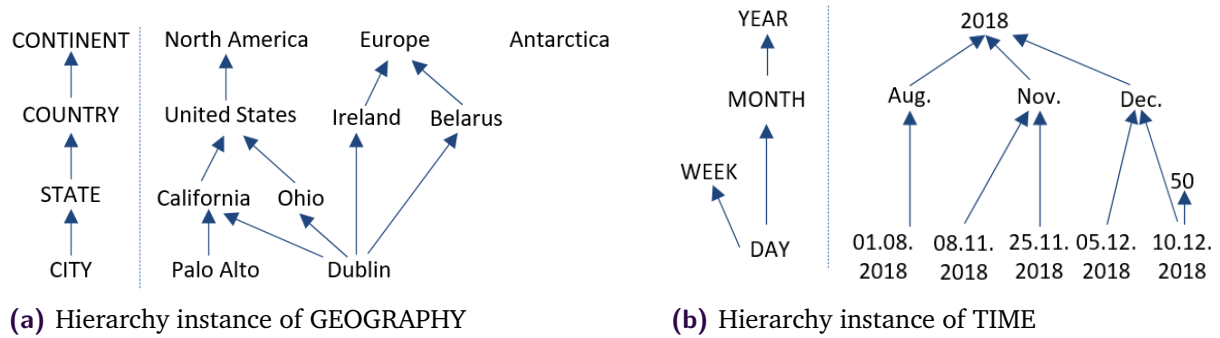
Figure 2.4.: Hierarchy instance examples
