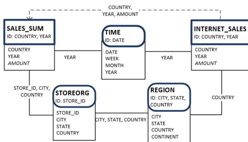
Figure 5.4.: Schema matchings between source schemas
