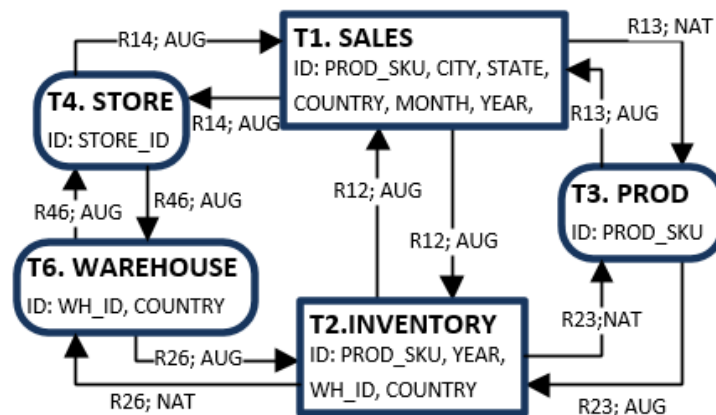
Figure 4.2.: SC graph example for Figure 2.9
