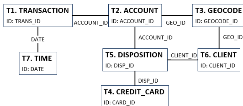
Figure 6.11.: Relationships for the bank retail database
