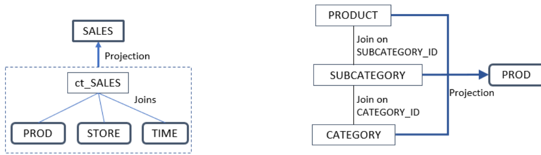
(a) Fact table SALES
