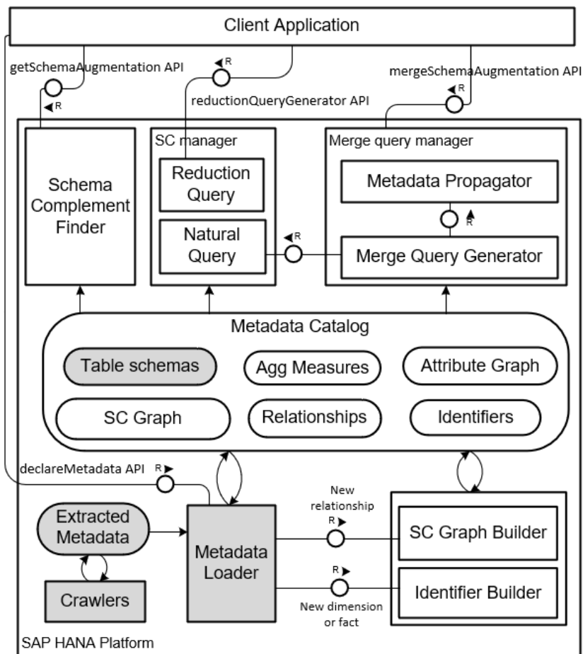
Figure 4.1.: Architecture overview
