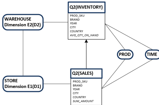
(a) Integration using dimensions E1(D1) and E2(D2)
