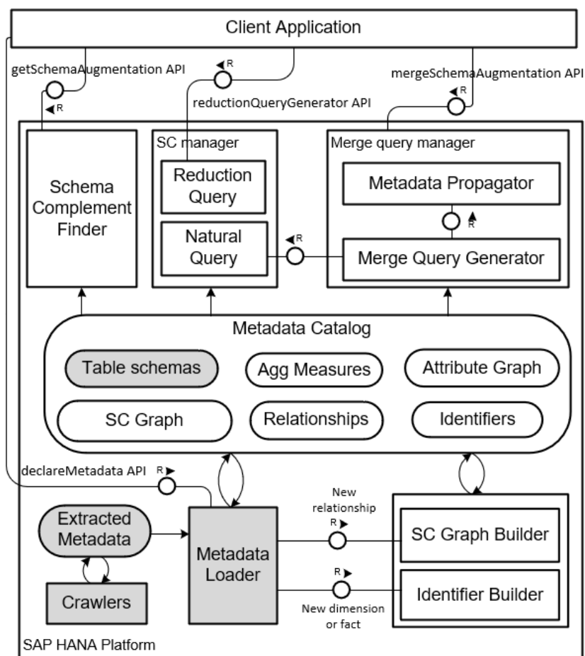
Figure 4.1.: Architecture overview
