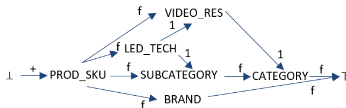
Figure 5.10.: Attribute graph of PROD_NEW
