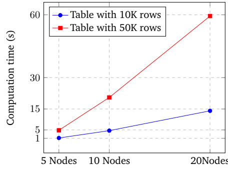
Figure 6.2.: Computation time for different number of nodes
