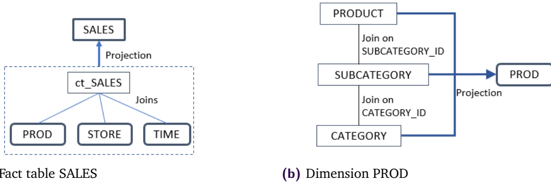
Figure 2.1.: Examples of definitions of analytic tables
