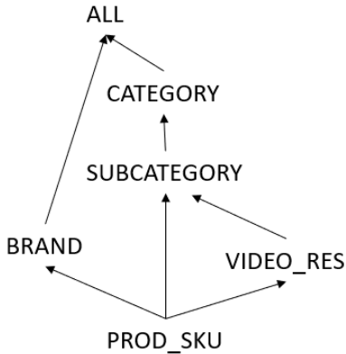
(a) Hierarchy type of PROD_NEW
