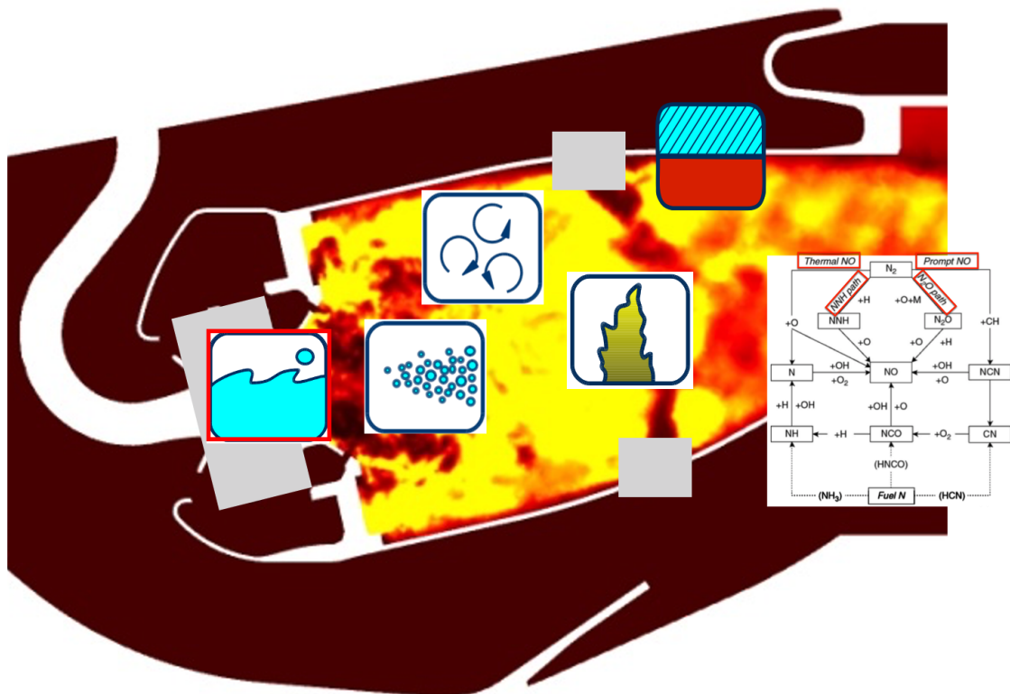
Figure 1: Representation of an aeronautical combustor, in which many physical phenomena take place: atomization, droplet transport, evaporation, turbulent mixing and combustion.
