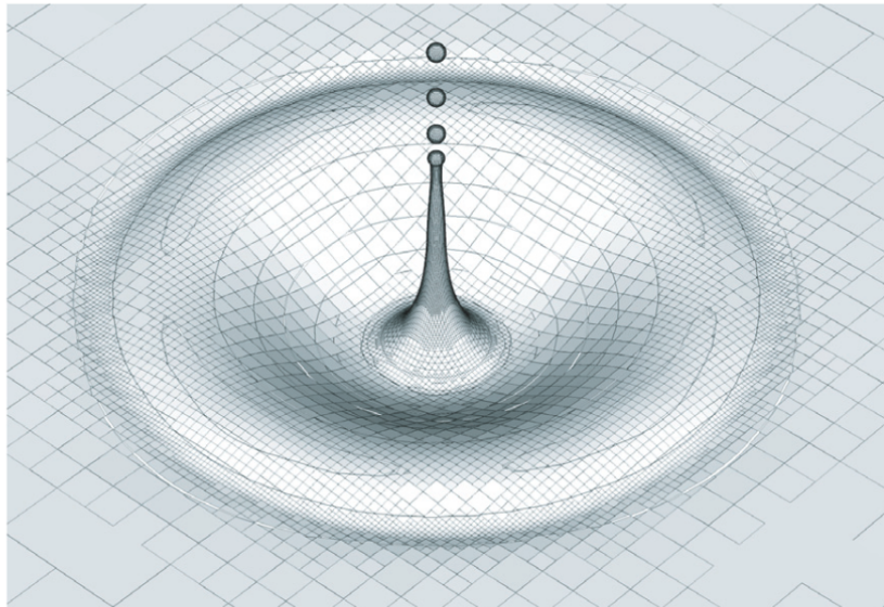
Figure 1.5: Jet created by the collapse under surface tension of an air bubble just below the surface of still water: the resolution varies along the interface according to local interface curvature. Reprinted from [75].
