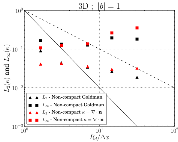
Figure 3.5: L_2 and L_\infty norms of the 3D interface curvature \kappa_\Gamma , using Goldman's formula and the classical formula, both discretized with non-compact stencils. The dashed and solid lines are first and second-order convergence, respectively.
