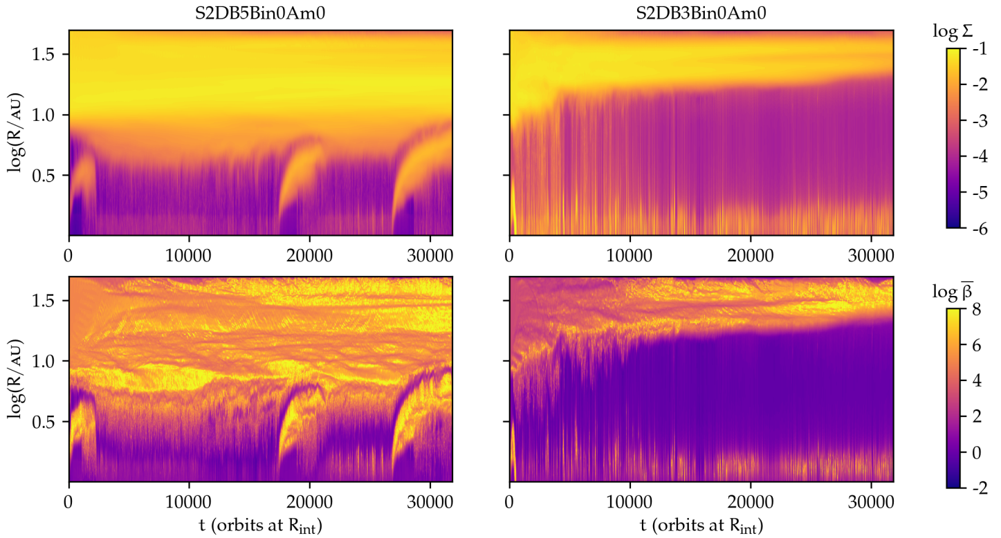
Figure 42: Spatio-temporal diagrams for \Sigma and \bar{\beta} for S2DB5BinoAmo (left panels) and S2DB3BinoAmo (right panels).
