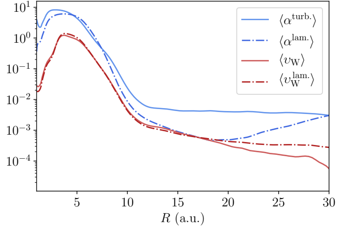
Fig. D.1. Time-averaged transport coefficients and their laminar and turbulent contributions. We give the laminar and turbulent contributions for \langle \alpha \rangle and the total profile with its laminar contribution for \langle \nu_W \rangle .
