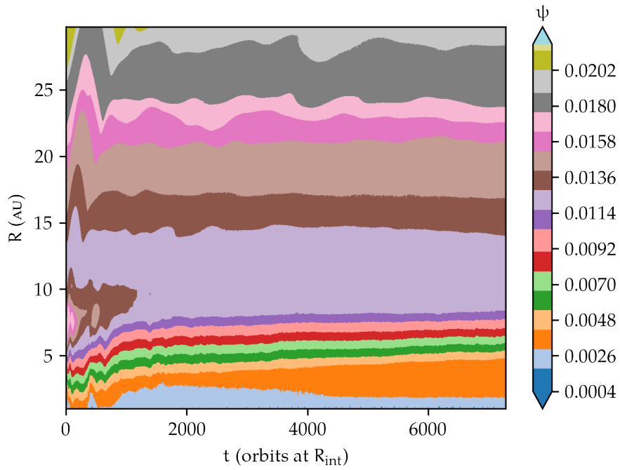
Figure 60: Magnetic field transport illustrated with the flux function \psi for the 3D fiducial simulation.
