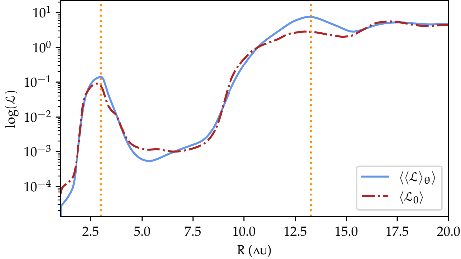
Figure 71: Characteristic function \mathcal{L} , theta and time-averaged in full blue line and taken at midplane and time-averaged in semi-dashed red line. The yellow dotted vertical lines mark the maxima of \mathcal{L} , at r_1 = 2.99 AU and r_2 = 13.2 AU.
