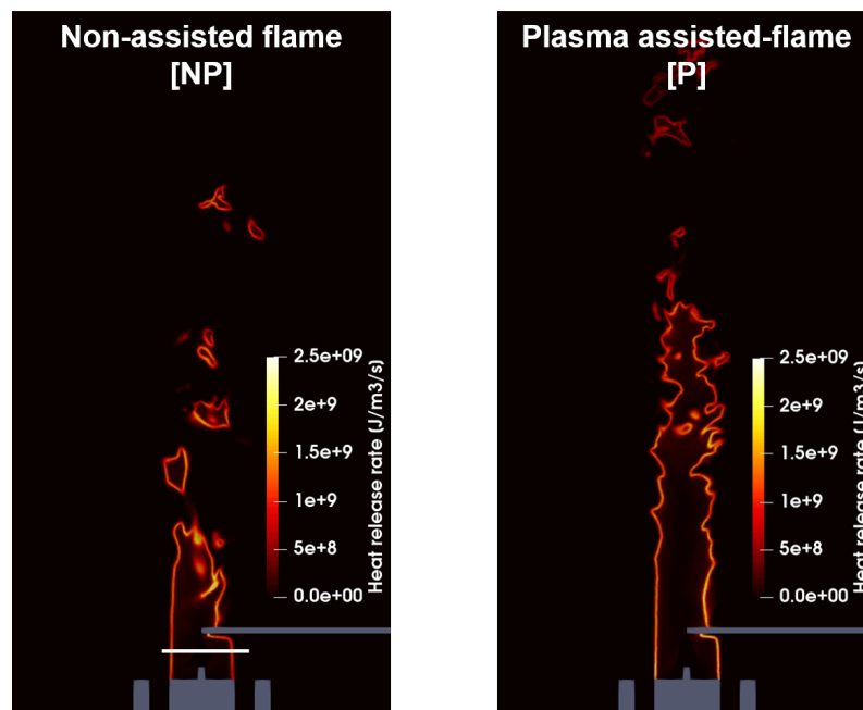
Figure 10.3: Instantaneous snapshots taken at the same time instant t=15 ms of the heat release rate for non-assisted flame case NP (left) and plasma-assisted flame case P (right). The white line shows the position of radial profiles represented in the following plots, 4.5 mm above the bluff body.
