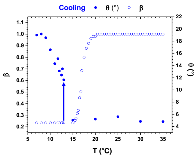
Figure 12: Contact angle and normalized transmitted light intensity versus temperature in a solution containing 1.2 mol/L NaCl and 16 mmol/L SDS. In the range between 15 and 13°C, the contact angle presents an abrupt increase on a time scale of the order of seconds.
