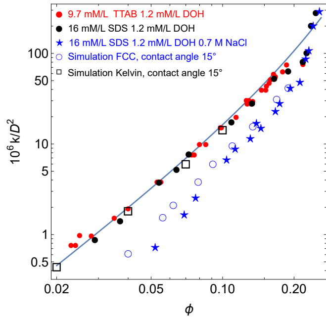
Fig. 8 Permeability of monodisperse foam scaled by the square of the bubble diameter D versus liquid volume fraction. The disk symbols represent data for foams with rigid interfaces: the red ones were obtained by Lorenceau et al 17 for foams with a bubble diameter D = 200\mu and the ionic surfactant TTAB. The black disks represent our data where the bubble diameter is D = 600\mu with the ionic surfactant SDS. In both cases, the co surfactant dodecanol (DOH) was added. Green stars represent our results where NaCl was added to induce attractive interactions, with a contact angle of 15^\circ . Open symbols are predictions for the permeability in the presence of attraction, derived from Surface Evolver simulations assuming a contact angle of 15^\circ , for either a face centered cubic or a Kelvin (body centered cubic) bubble packing structure, as described in the text.
