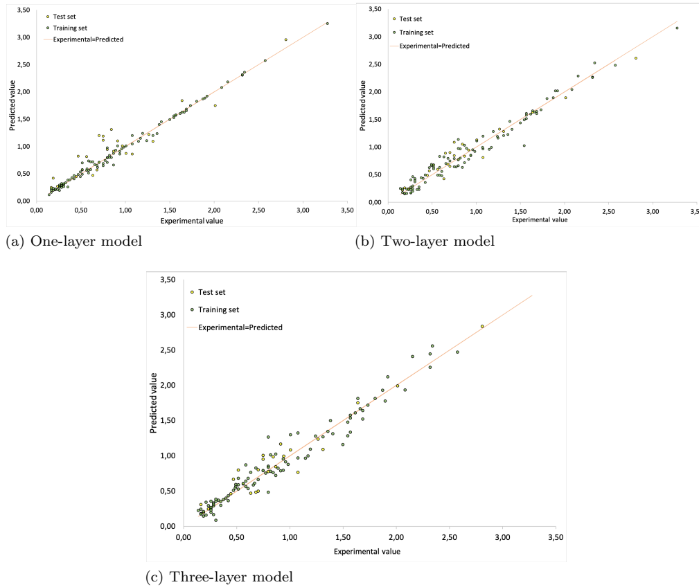
Figure 6.5: Flexural strength prediction versus experimental value on the training and test set for one, two and three layer models
