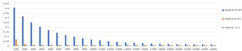
Figure 7.5: Variation of the cost function for a maximum of 2400 iteration with varying \alpha to Y_1 (lime)
