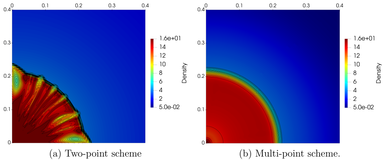
Figure 4.17: Noh implosion problem on polar grids — Density maps for a 200 \times 200 quadrilateral polar grid.
