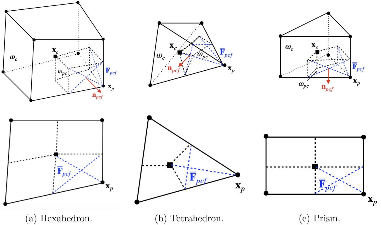
Figure 4.20: Geometrical entities attached to a cell \omega_c (top) and its subsurface fluxes partition of a face f of cell \omega_c (bottom).
