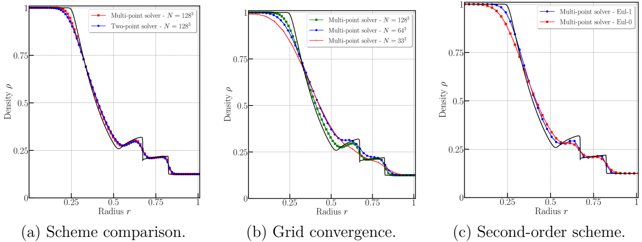
Figure 4.23: Spherical Sod shock tube — Comparison of numerical density with reference solution (black line) at t_{final} = 0.2
