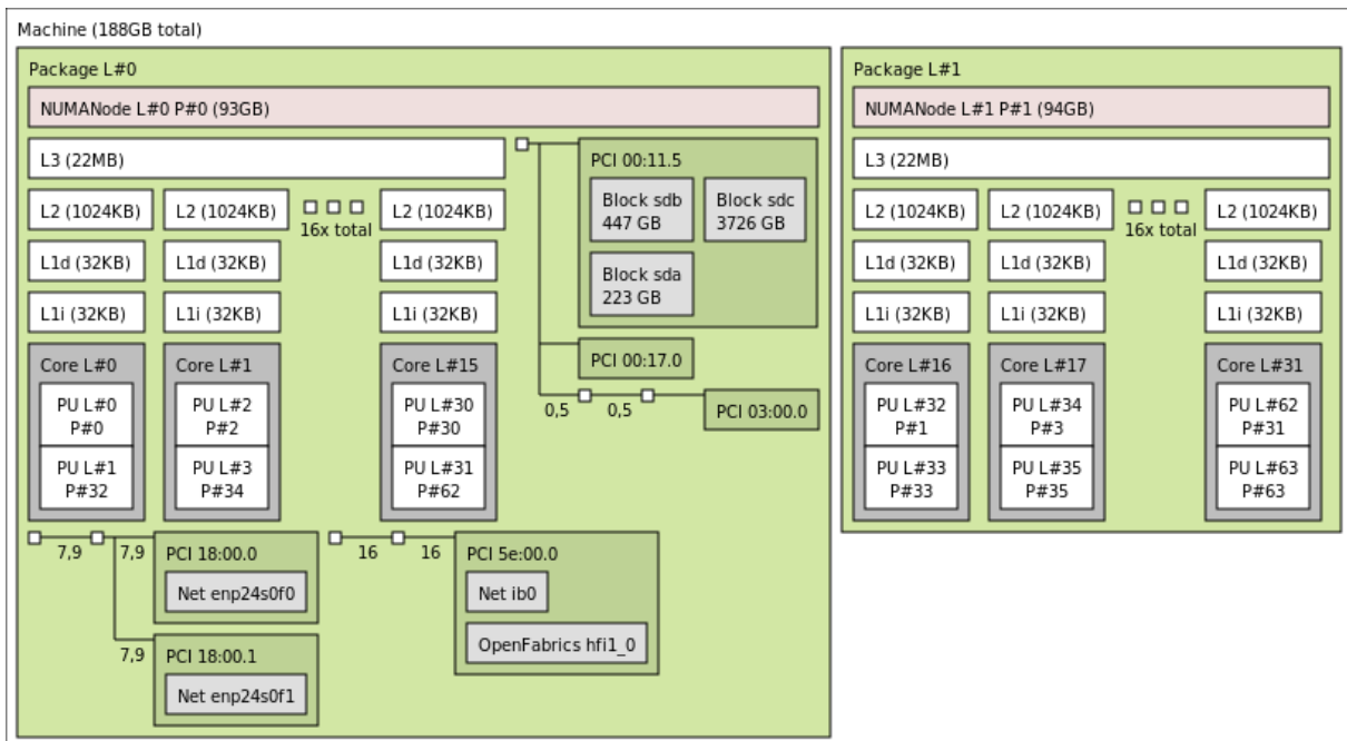
Figure C.3: dahu's topology.
