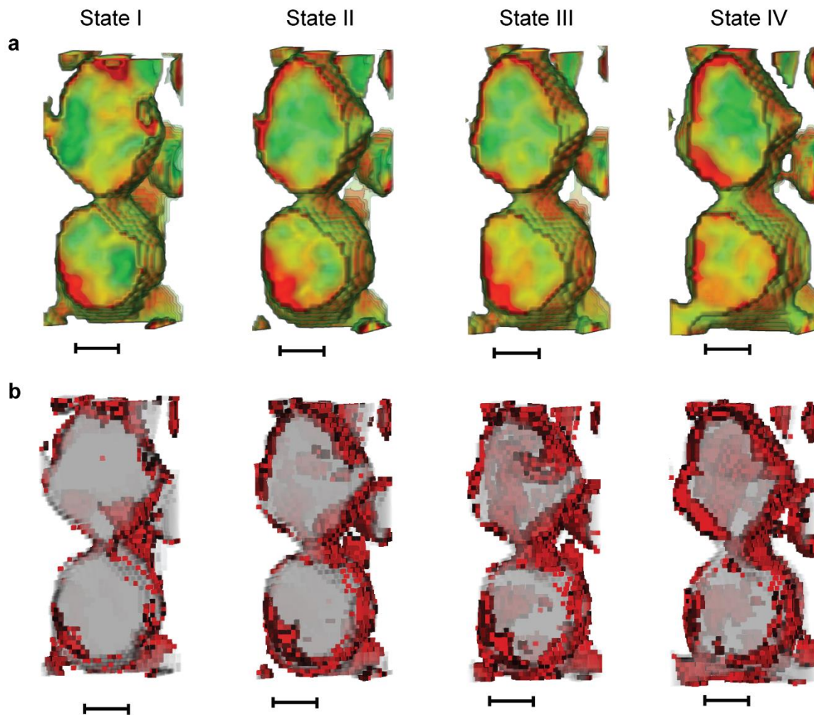
Figure VII-3. Zoom on the individual NMC secondary particles across the lithiation process. a. 3D map of Li concentration evolution as the lithiation proceeds. b. Repartition of the Li-rich regions (in red) at each state of lithiation (I-IV). The scale bars represent 2 \mu\text{m} .
