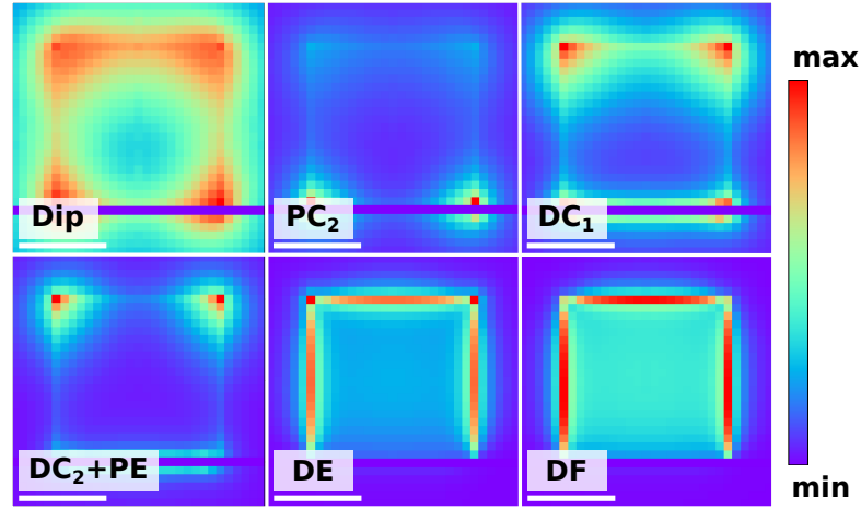
Figure 7.5: FDTD-simulated spectral maps for the cube-substrate system, including the dipolar (Dip), second proximal corner ( PC_2 ), first distal corner ( DC_1 ), second distal corner ( DC_2 ), proximal edge (PE), distal edge (DE), and distal face (DF) modes. Scale bars are 50 nm.
