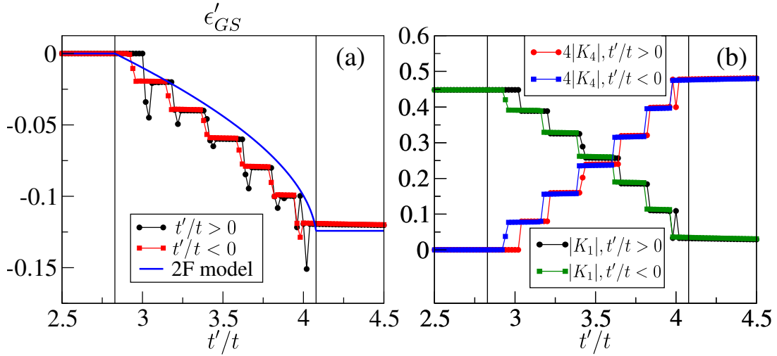
Figure 5.11: Energy observables in the ground-state of (5.1) with M = 4 on a lattice with L = 96 sites as a function of \left|\frac{t'}{t}\right| for both t' \leq 0 and t' \geq 0 . Vertical lines are transition points predicted by the generalized 2F model (5.4). (a) First derivative of the energy density with respect to \frac{t'}{t} from DMRG and 2F model (5.4). (b) Single-particle and tetramer kinetic energy densities K_1 and 4K_4 .
