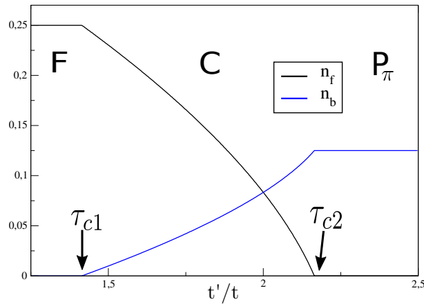
Figure 3.4: Optimal fermionic and bosonic densities obtained by minimizing \frac{E_2 F}{t} for a total density n = 0.25 . Two critical points, \tau_{c1} and \tau_{c2} , divide the phase diagram into three distinct phases: (i) the fermionic F phase, where the system is populated by fermions only, (ii) the C phase, characterized by the coexistence of fermions and hard-core bosons, and (iii) the P_\pi phase, where the system is populated by hard-core bosonic particles only.
