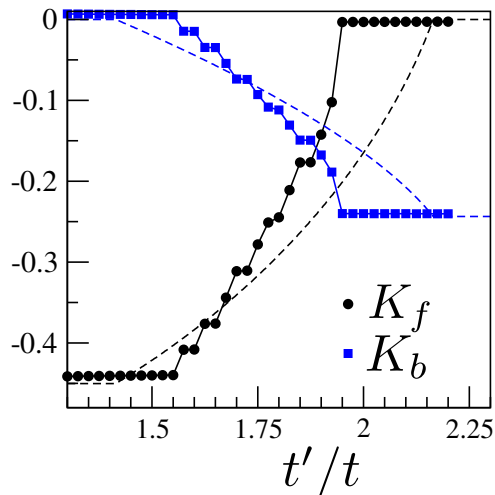
Figure 3.7: Total single-particle kinetic energy density K_f and pair kinetic energy density K_b , probing almost directly n_f and n_b . The black dotted line corresponds to the 2F model prediction for K_f , while the blue dotted line is the one for K_b . The sequence of small plateaus in K_f and K_b corresponds to the progressive formation of tightly-bound pairs when increasing the value of \frac{t'}{t} .
