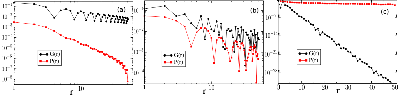
Figure 3.10: Decay of the (absolute value of the) single-particle correlator G(r) and of the pair correlator P(r) (a) in the F phase ( \frac{t'}{t} = 1.4 ), (b) in the C phase ( \frac{t'}{t} = 1.8 ) and (c) in the P_\pi phase ( \frac{t'}{t} = 2.0 ) for a system of size L = 104 in OBC and at filling n = 0.25 .
