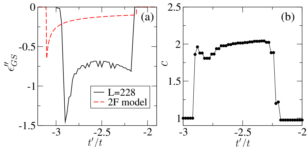
Figure 5.5: (a) Second derivative of the ground-state energy density e''_{GS} with respect to \frac{t'}{t} for the Hamiltonian in Eq. (5.1) (continuous line) and for the model \hat{H}_{2F} (dashed line). (b) Central charge c as a function of \frac{t'}{t} .
