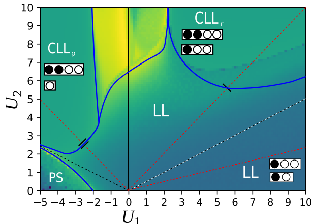
Figure 2.8: Phase diagram for n = \frac{2}{5} . The color map for the background displays the half-chain entanglement entropy on a system with L = 30 and PBC. Black lines are classical transition lines obtained neglecting quantum fluctuation. Additional numerical simulations are presented for the points lying on the red lines. Blue lines are a guide to the eye for the main phase boundaries.
