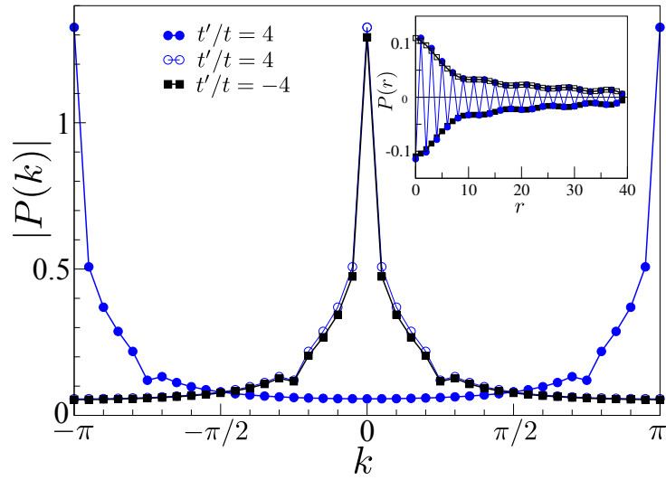
Figure 3.3: Absolute value of the Fourier transform of pair correlations for an open chain with L = 80 and \frac{t'}{t} = \pm 4 . Open symbols are the \frac{t'}{t} = 4 data shifted by \pi . Inset: Pair correlations.
