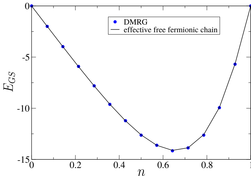
Figure 5.1: DMRG ground state energy E_{GS} = N\epsilon_G S for M = 3 and L = 42 sites with PBC with t' = 1 and t = 10^{-4} as a function of the filling n and compared with the analytical expression provided in Eq. (5.3).
