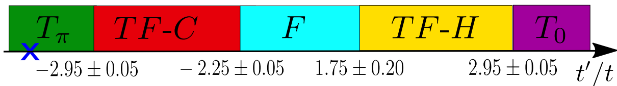
Figure 5.3: Phase diagram of the model in Eq. (5.1) in the case M = 3 (not in scale).
