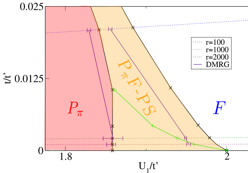
Figure 4.11: Phase diagram in the \frac{t}{t'} \rightarrow 0 limit. Black lines are the boundaries of the P_\pi F - PS phase obtained from model (4.14) for several values of the radius r . Violet lines are DMRG estimates of the phase boundaries for r = 100, 1000, 2000 . The green line sketches the boundary between the phase separation regime with a fermionic CDW domain (below the line) and the one with a fermionic liquid domain (above the line).
