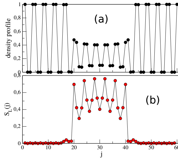
Figure 2.11: DMRG results for n = \frac{2}{5} along the U_1 = 0 line for U_2 = 20 , L = 60 and PBC. (a) Density profile. (b) Entanglement entropy profile S_L(j) .
