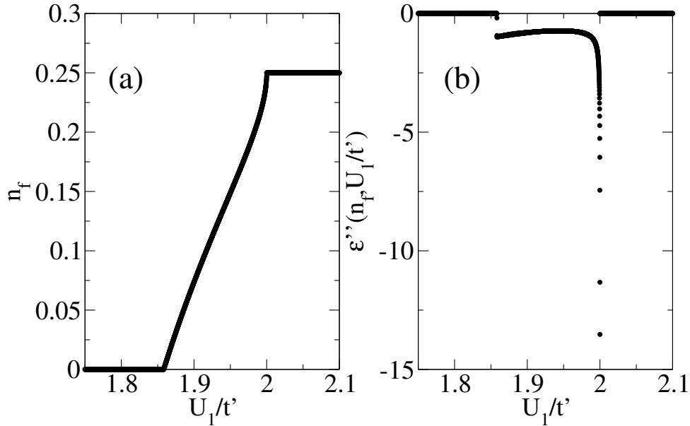
Figure 4.10: (a) Optimal fermionic density n_f(\theta) as a function of \tan \theta = \frac{U_1}{t} according to the effective phase separation model (4.12). (b) Second derivative of the energy density \mathcal{E}(n_f(\theta), \theta) in Eq. (4.12) as a function of \tan \theta = \frac{U_1}{t} .
