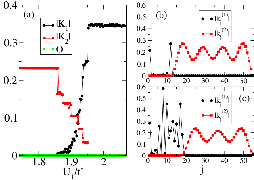
Figure 4.7: Cut showing the P_\pi F - PS phase for a chain with L = 56 and PBC. In this small t limit, we fix \frac{t}{t'} = \frac{1}{2000} \sqrt{1 + (\frac{U_1}{t'})^2} . (a) Kinetic energies K_1 , K_2 and overlap O as a function of \frac{U_1}{t'} . (b) Local kinetic energy profiles k_j^{(1)} and k_j^{(2)} for \frac{U_1}{t'} = 1.891646 , indirectly showing a CDW fermionic domain. (c) Same for \frac{U_1}{t'} = 1.912426 , without CDW domain.
