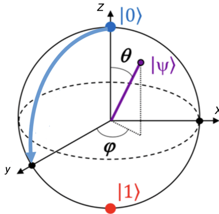
FIGURE 2.1: Bloch sphere
