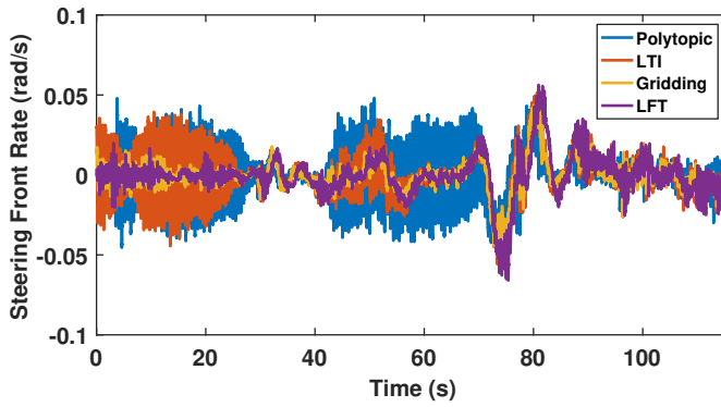
FIGURE 4.24: Experimental steering front rate of the LTI and LPV controllers ( rad/s )
