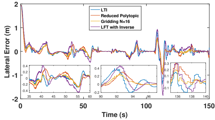
FIGURE 4.17: Lateral error for robustness comparison (m)
