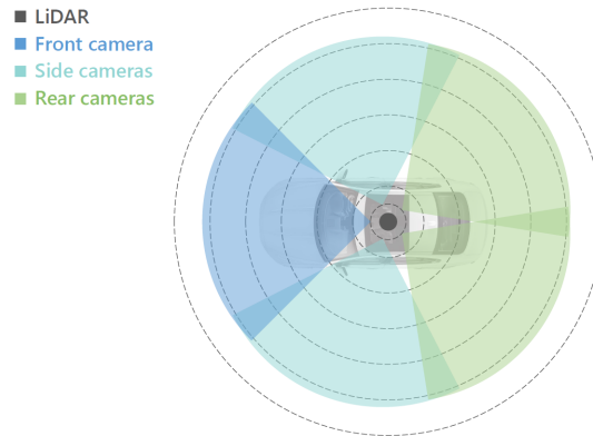
FIGURE 3.4: Sensor setup in the automated ZOE Vehicle [318]
