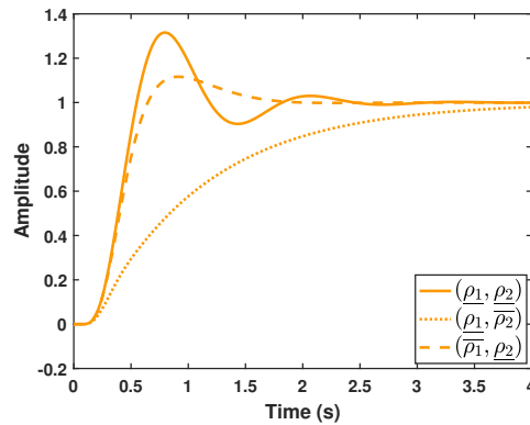
FIGURE 6.13: Closed-loop step response with K^{(0)}(\rho)
