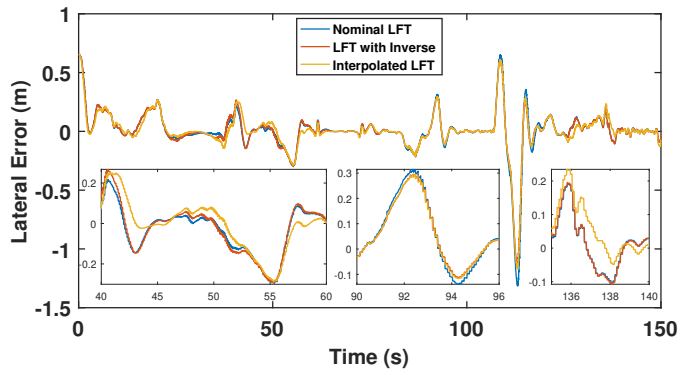
FIGURE 4.15: Lateral error using the LFT approaches ( m )
