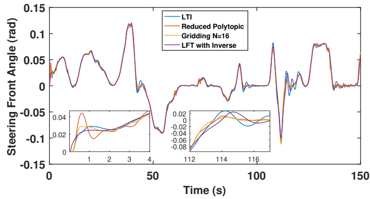
FIGURE 4.18: Steering front angle for robustness comparison (m)
