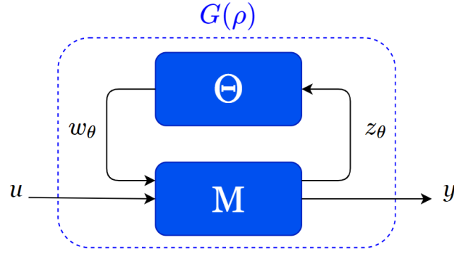
FIGURE 4.3: Linear fractional representation of a parameter-varying system
