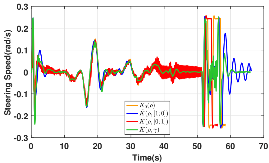
(C) Steering speed \dot{\delta} (rad/s)
