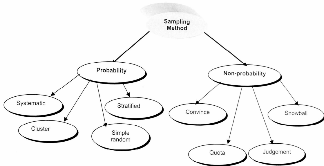
Figure C4.3: Sampling methods
