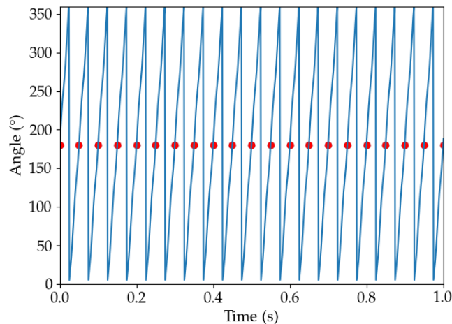
Figure A.1: Position measurement of a PISTIL rotation configured at 7200^\circ \cdot s^{-1} (20 Hz rotation)
