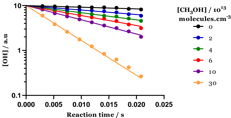
Figure 48: OH fluorescence signal (logarithmic scale) as a function of reaction time for [H] = 5 \times 10^{11} molecules cm^{-3} , [NO_2] = 1 \times 10^{13} molecules cm^{-3} , and [CH_3OH] = 0 - 30 \times 10^{13} molecules cm^{-3}
