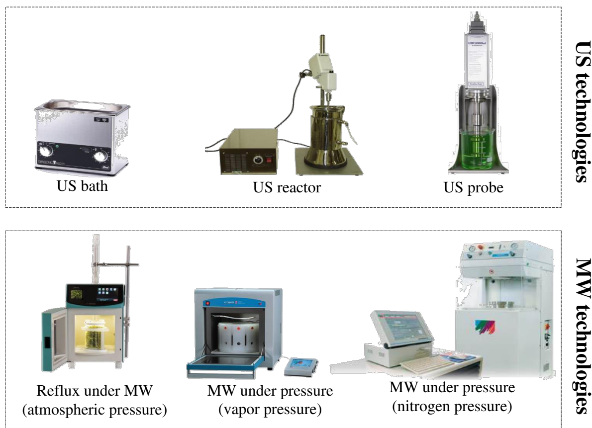
Figure II-4. Equipments assessed for the ultrasound and microwave assisted extraction study.
