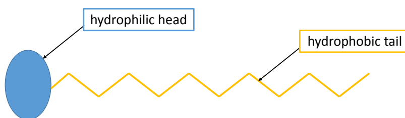
Figure I-13. Surfactant/hydrotrope structure.
