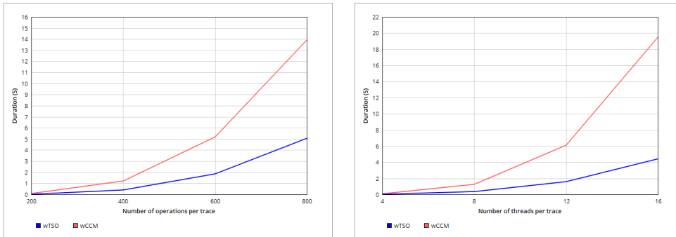
(a) Checking wTSO and wCCM while varying the number of operations. (b) Checking wTSO and wCCM while varying the number of cpus.
