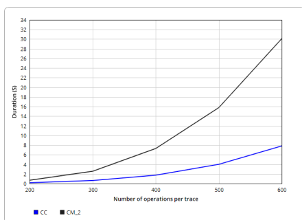
(e) Comparing CM_2 and CC violations runtimes while varying the number of operations.
