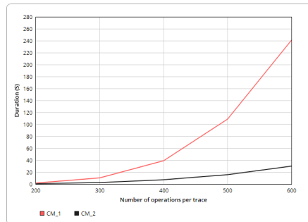
(d) Comparing CM_1 and CM_2 runtimes while varying the number of operations.
