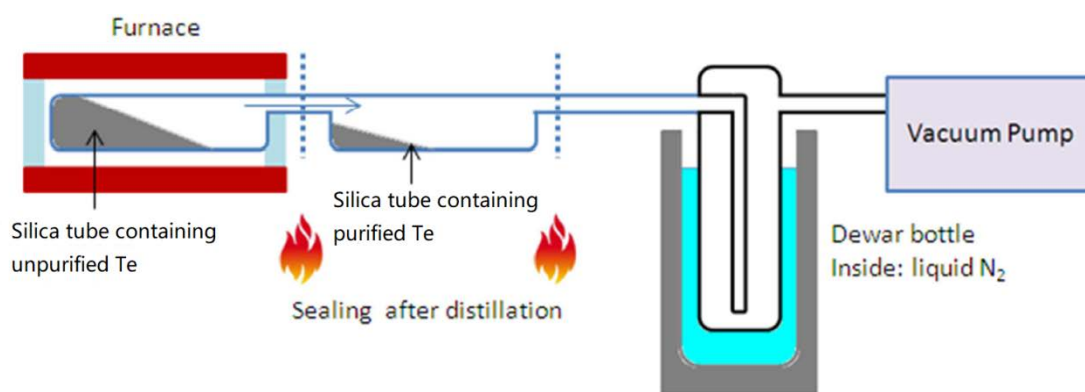
Figure 3.2 Schematic explanation of tellurium purification
