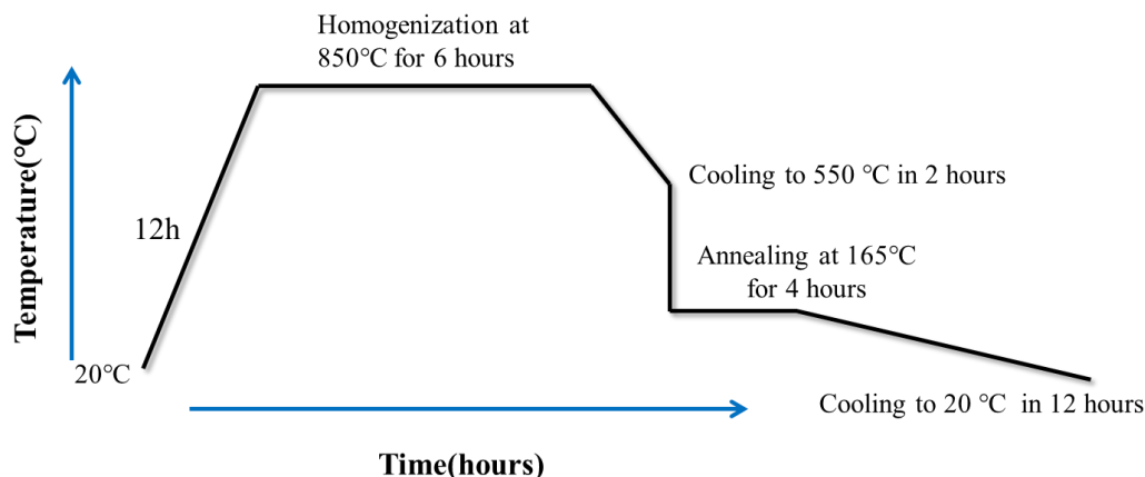
Figure 3.26 Program set for the homogenization of \text{As}_{38}\text{Se}_{62} glass
