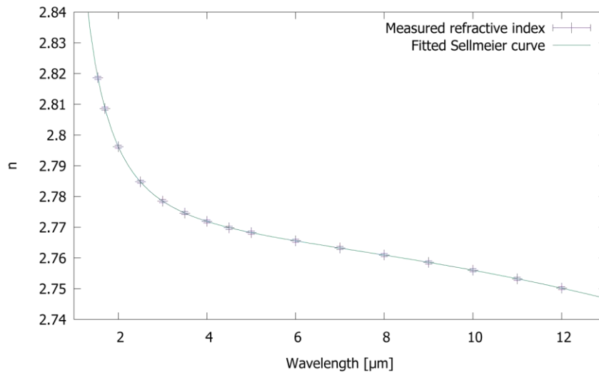
Figure 3.22 Measurement of the refractive index of \text{As}_{38}\text{Se}_{62} compared to fitted Sellmeier curve
