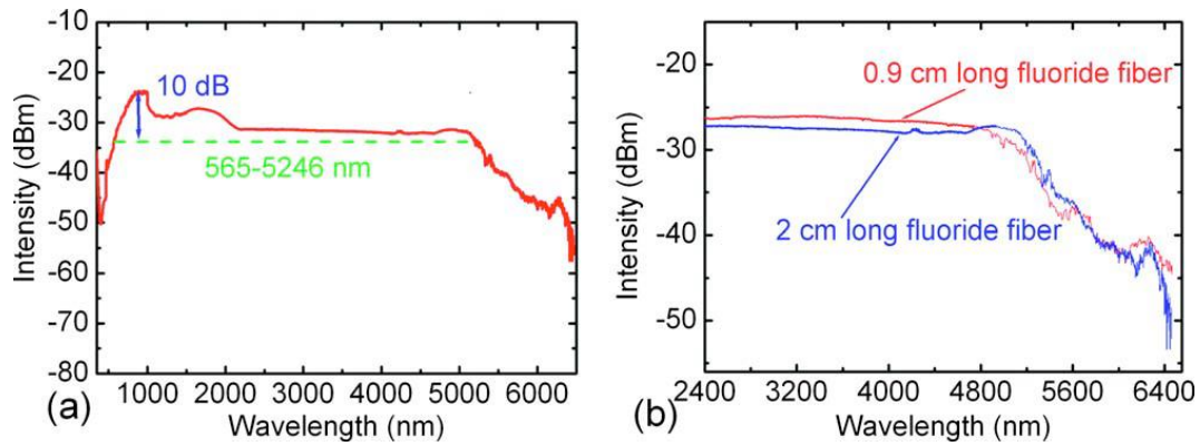
Figure 1.5 (a) The measured SC spectra from the 2-cm-long fluoride fiber when the average pump power of 1450\text{ nm} femtosecond laser was fixed at 20\text{ mW} (the corresponding peak power is about 50\text{ MW} ) (b) A comparison of the long-wavelength edge of SC spectra in 0.9 or 2\text{ cm} long fluoride fiber [51]
