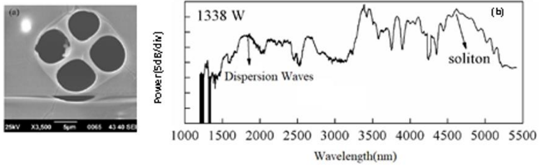
Figure 1.13 (a) Cross section of the AsSe 2 –As 2 S 5 hybrid MOF. (b) Output spectrum of the mid-infrared supercontinuum obtained by pumping at 3389 nm[94]
