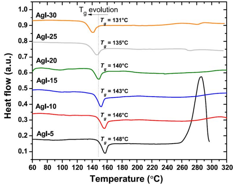
Figure 3.1 DSC curves of the (\text{Te}_4\text{Ge})_{100-x}(\text{AgI})_x glasses ( x=5, 10, 15, 20, 25 , and 30).
