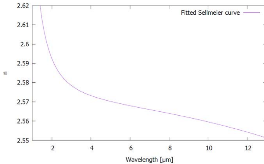
Figure 3.23 Fitting of the Sellmeier curve of \text{Ge}_{10}\text{As}_{22}\text{Se}_{68} glass
