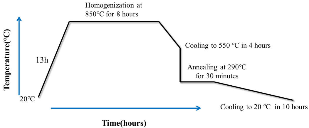
Figure 2.3 Thermal profile of the synthesis of \text{Ge}_{20}\text{As}_{20}\text{S}_{60} glass
