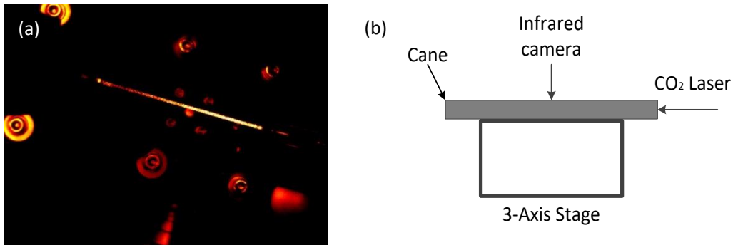
Figure 3.36 (a) Infrared image of light scattering from the side of the cane (b)
