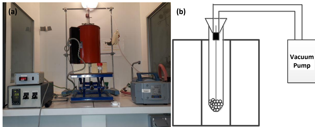
Figure 3.41 (a) Experimental setup of the filling of chalcogenide in to silica PCF
