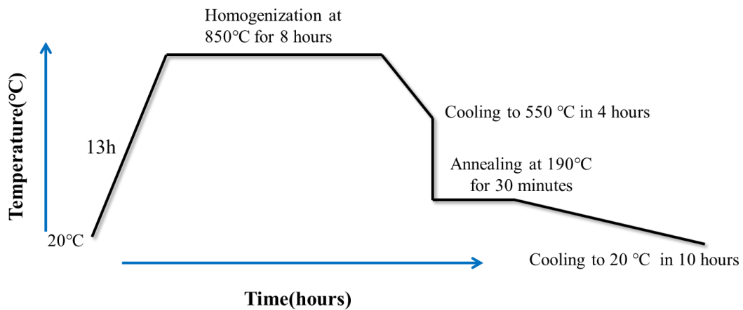
Figure 2.2 Thermal profile of the synthesis of \text{Ge}_{15}\text{As}_{15}\text{S}_{70} glass
