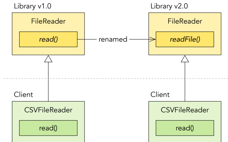
Figure 8.3: In v1.0, library used to provide an abstract hook read() that was meant to be implemented by clients. In v2.0, this hook was renamed to readFile() . But the client system still provides the implementation for the old method read() . Now the client implementation will never be called.
